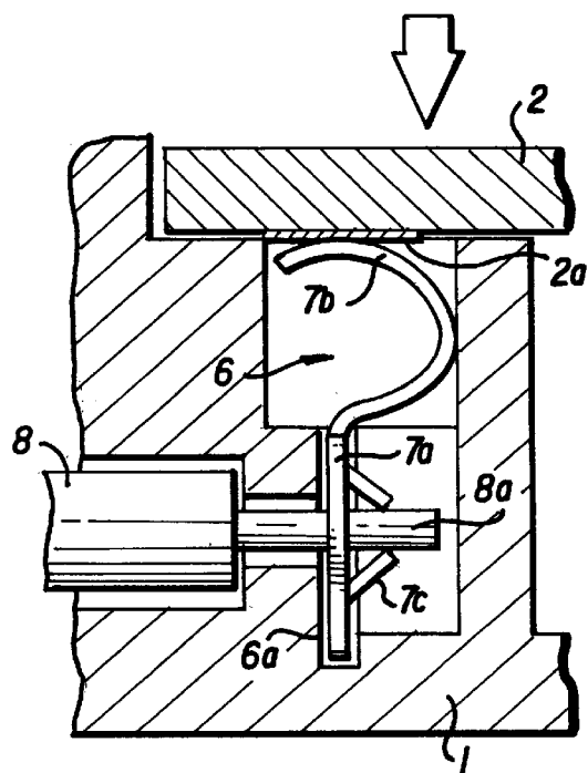
FIG. 6 (PRIOR ART)
