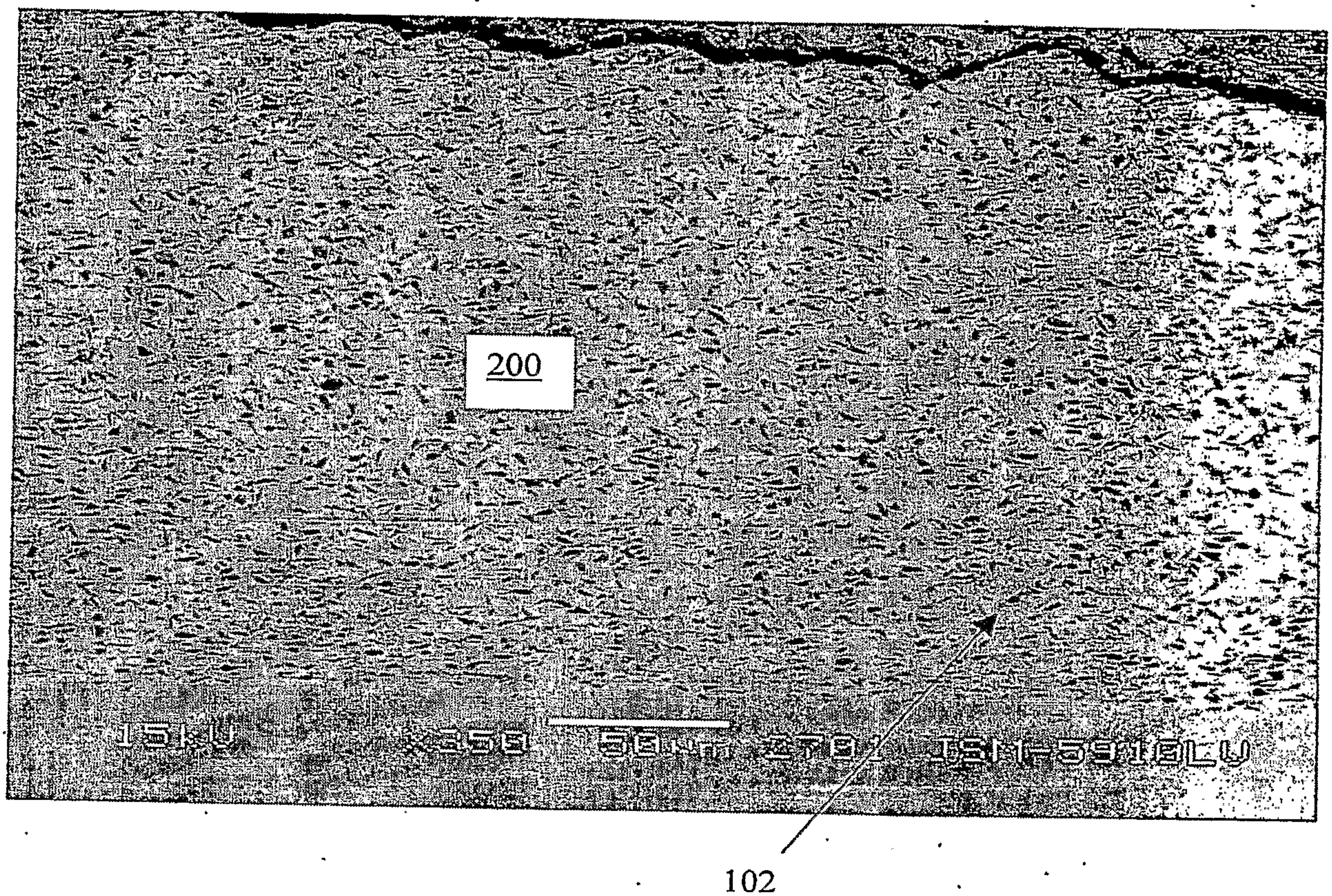
Fig. 2 D.C. electroplated Co - P- SiC electrocomposite coating
