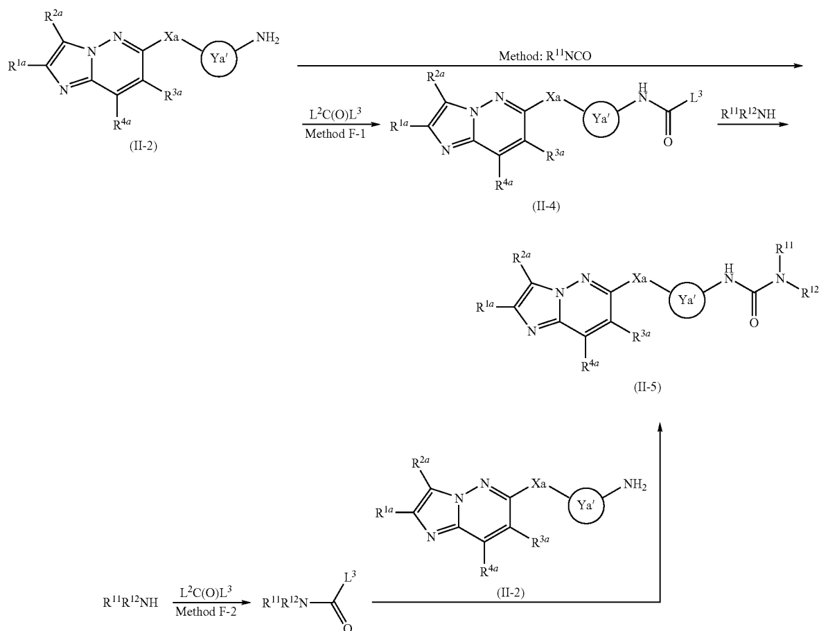
(Scheme 3)
