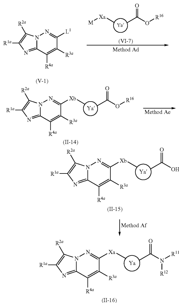
(Scheme 12)
