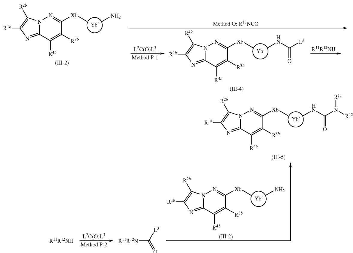
(Scheme 8)
