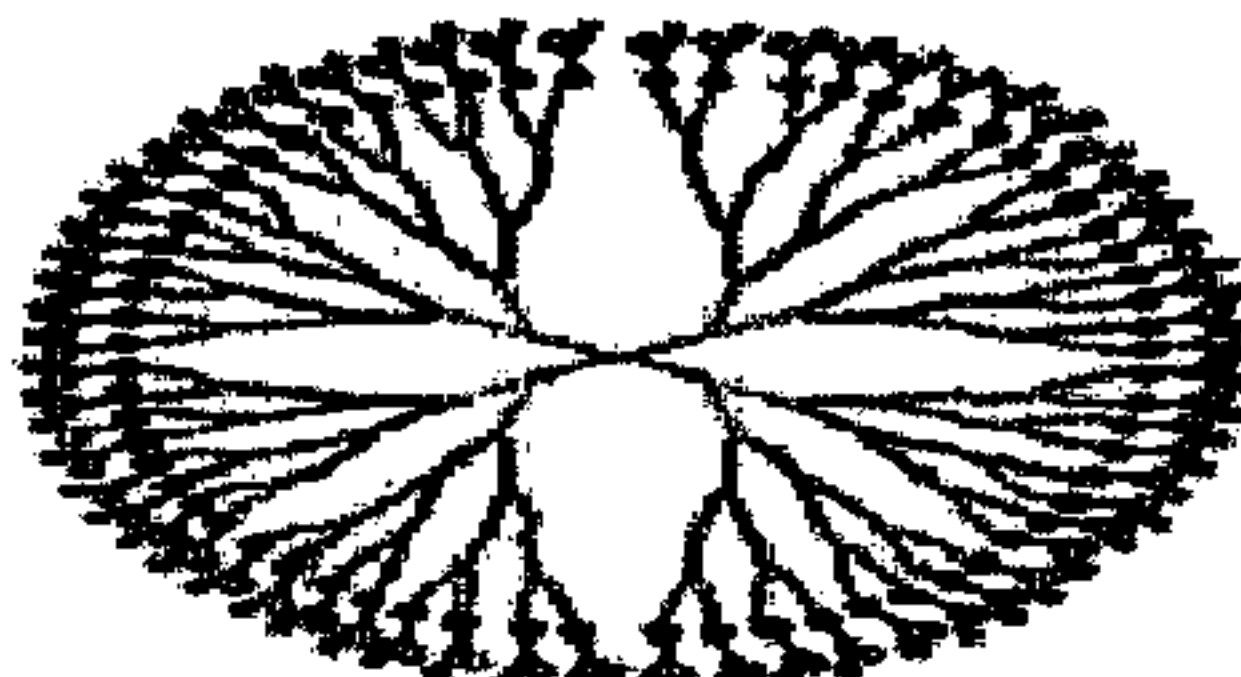
Bifunctional G4-PAMAM dendrimer ● = NH 2 ○ = SH, or OH, or COOH } Total of \geq 110 functionality
