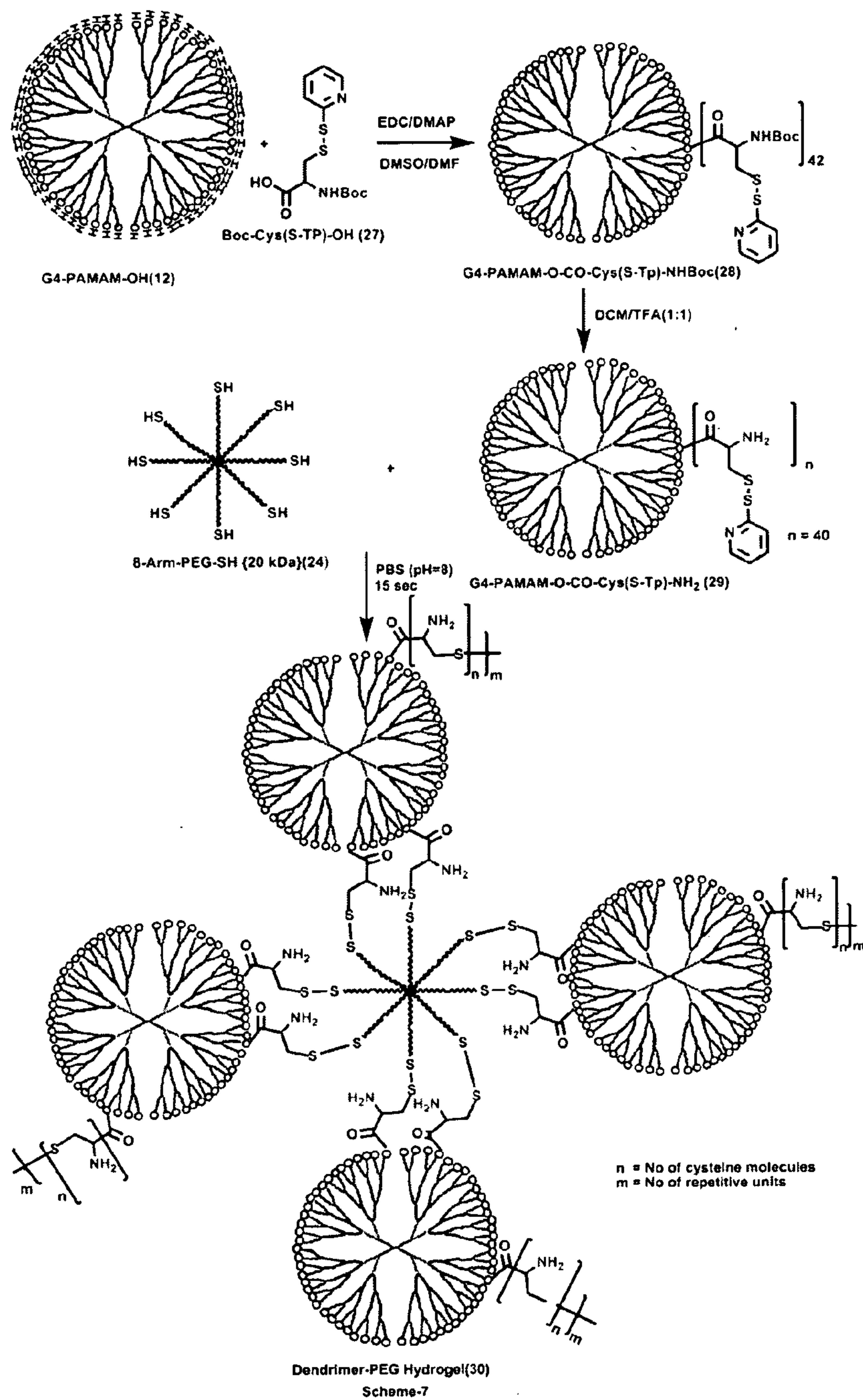
Scheme 7. Schematic representation for the formation of hydrogel involving one of the functional handles of the G4-PAMAM-O-CO-Cys(S-TP)-NH 2 dendrimer while the 'NH 2 ' handle is available for further modifications. The thiol terminated 8arm PEG (20 kDa)
