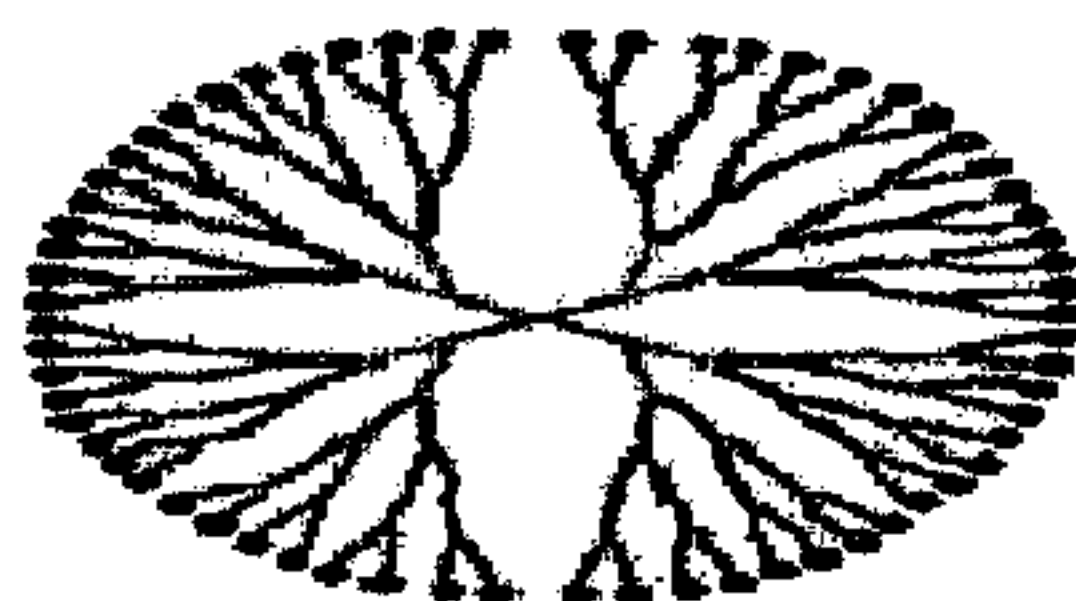
G4-PAMAM ● = OH, COOH, NH 2
