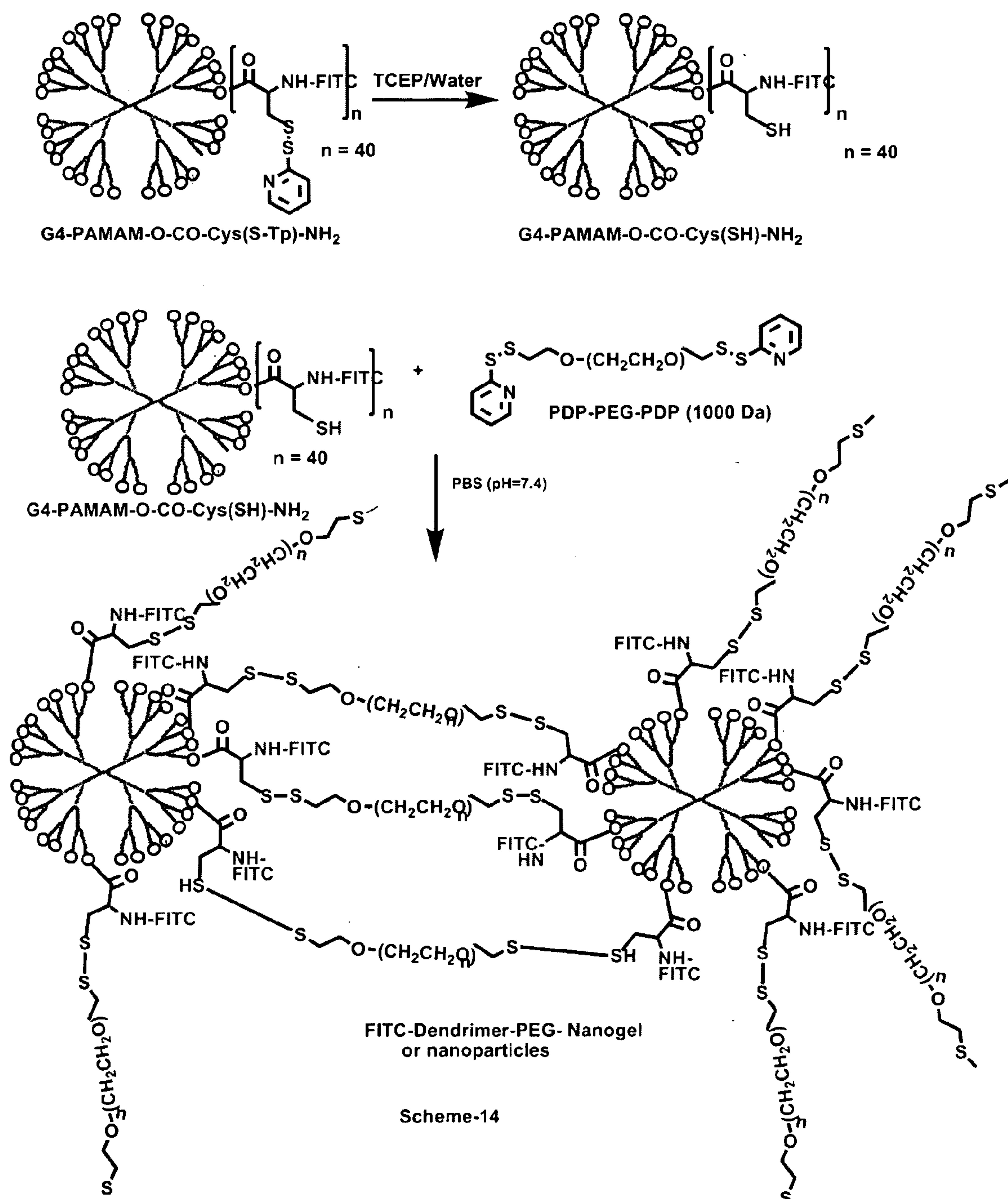
Scheme-14: G4-O-CO-Cys(SH)-NH 2 cross linked with PDP-PEG-PDP to form dendrimer-PEG nanogel (or nanoparticles)
