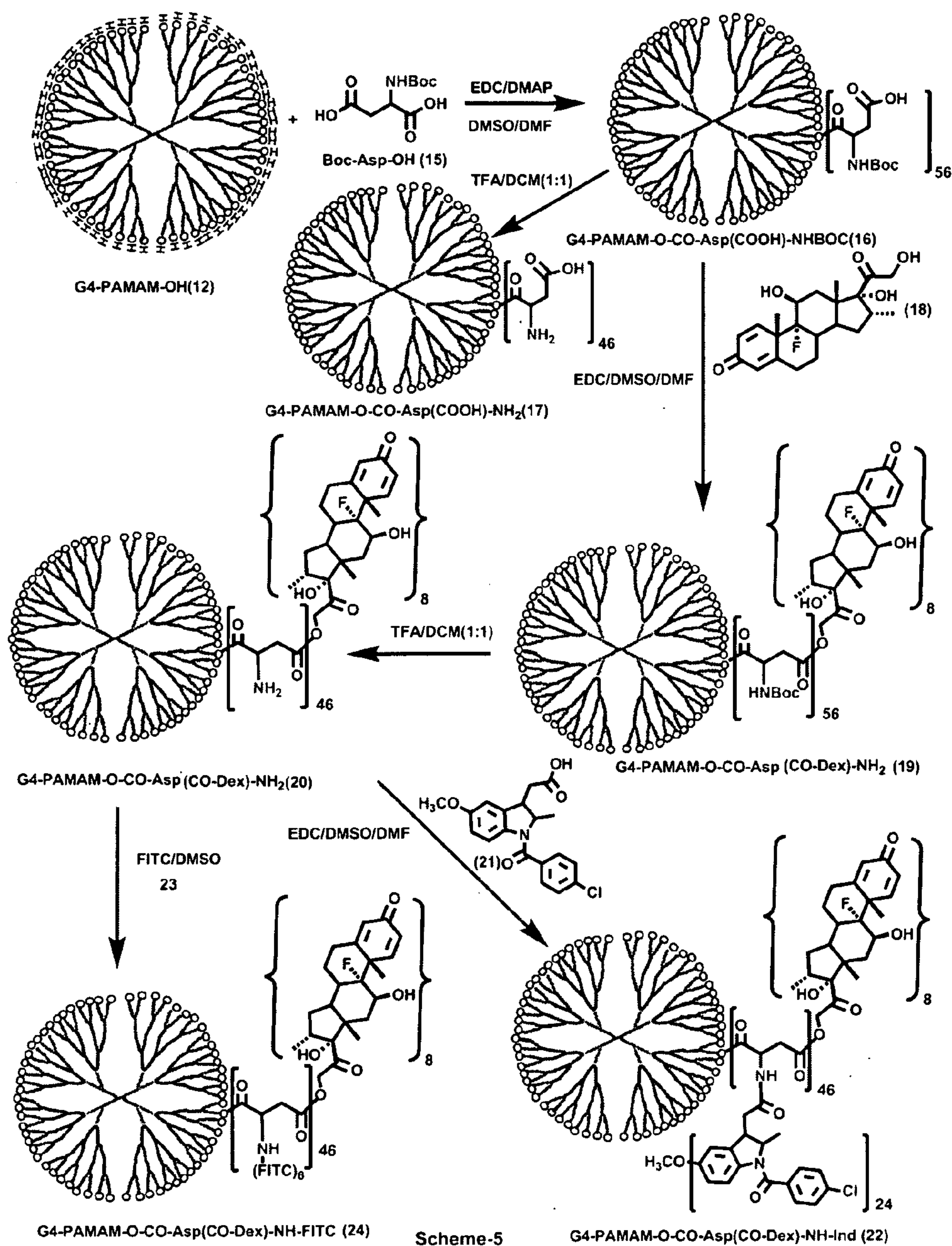
Scheme 5. Schematic representation for the post-functionalization reactions of hetero-bifunctional dendrimers showing conjugation of multiple drugs and or imaging agents in immediate succession. G4-PAMAM-O-Asp(COOH)-NH 2 (17) dendrimer bearing COOH and NH 2 termini was synthesized. Dexamethasone was conjugated to G4-PAMAM-O-Asp(COOH)-NH 2 (16) and indomethacin was added to achieve G4-PAMAM-O-Asp(CO-
