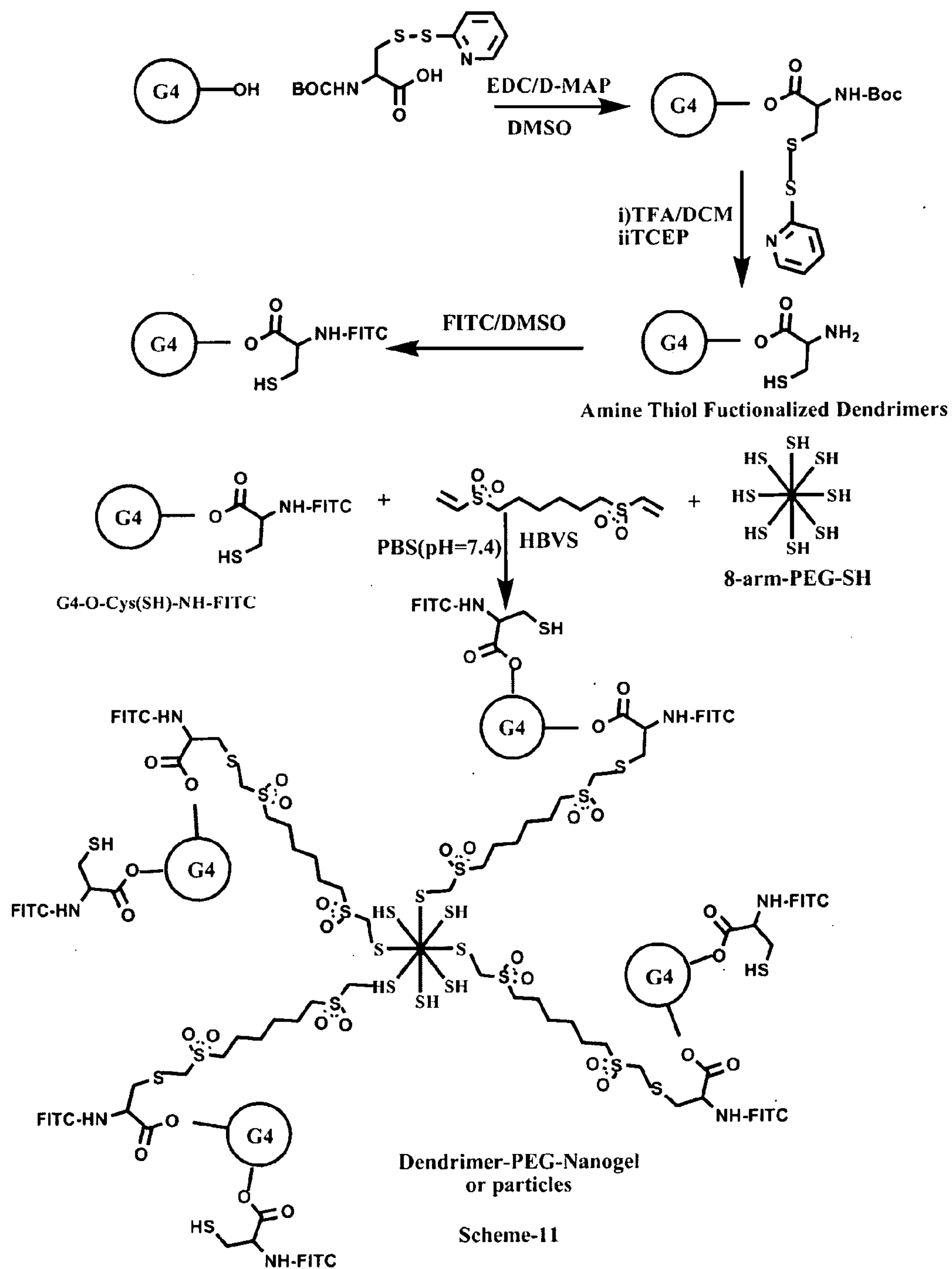
Scheme-11: HBVS cross linked with G4-O-Cys(SH)-NH-FITC and 8-arm-PEG-SH to form dendrimer-PEG nanogel (or nanoparticles)
