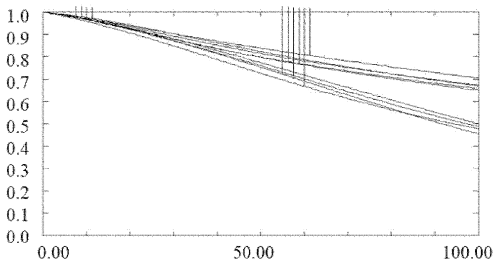
Modulation Transfer Function, MTF
