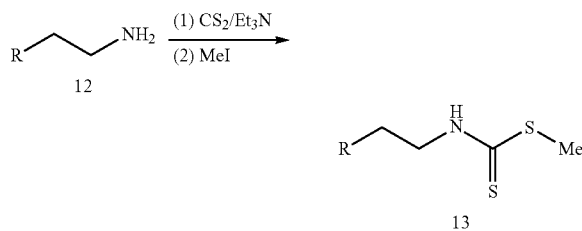
Scheme 5. General procedure for synthesis of targets in series 5
