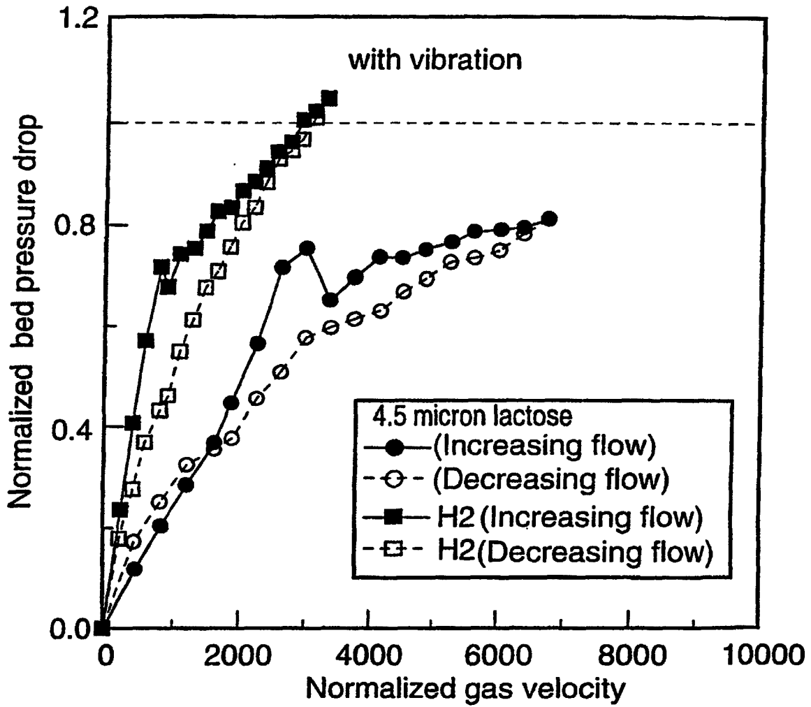
Normalized bed pressure drop vs. normalized superficial gas velocity for 4.5 \mu\text{m} lactose powder (with vibration)
