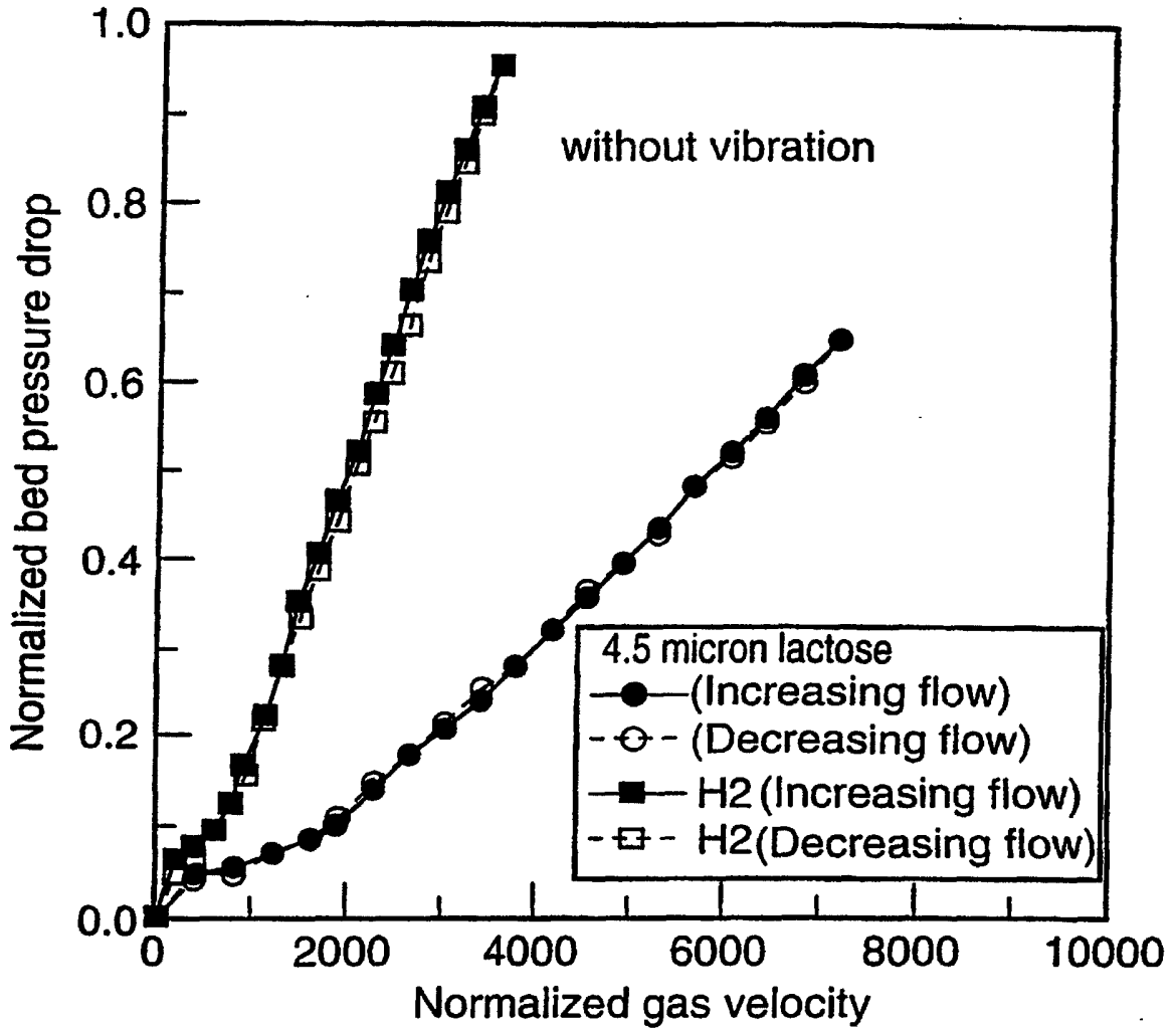
Normalized bed pressure drop vs. normalized superficial gas velocity for 4.5 \mu\text{m} lactose powder (without vibration)
