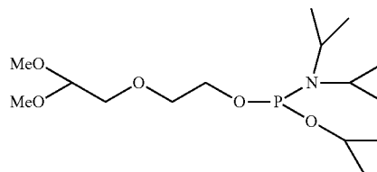
2-(2,2-Dimethoxy-ethoxy)-ethanol
