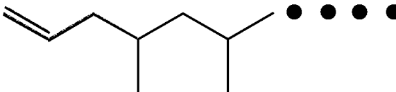
allylic vinyl end group
