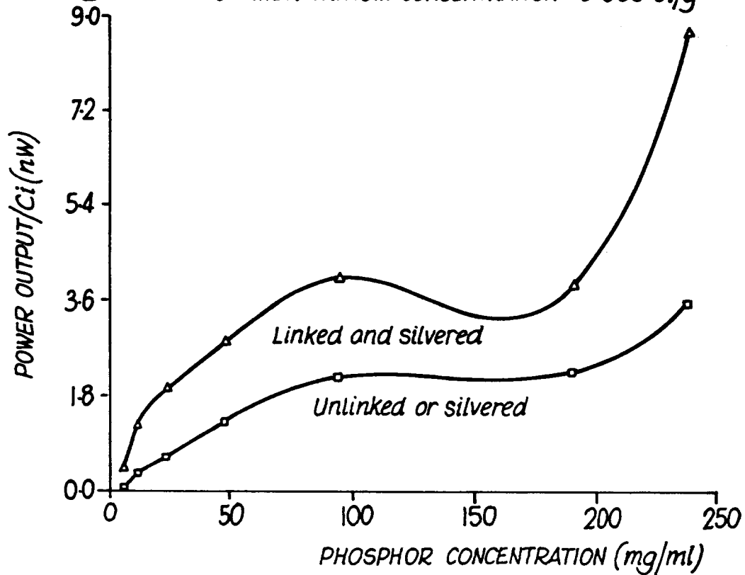
Fig.3. POLYMER TRITIUM CONCENTRATION 0.606 Ci/g
