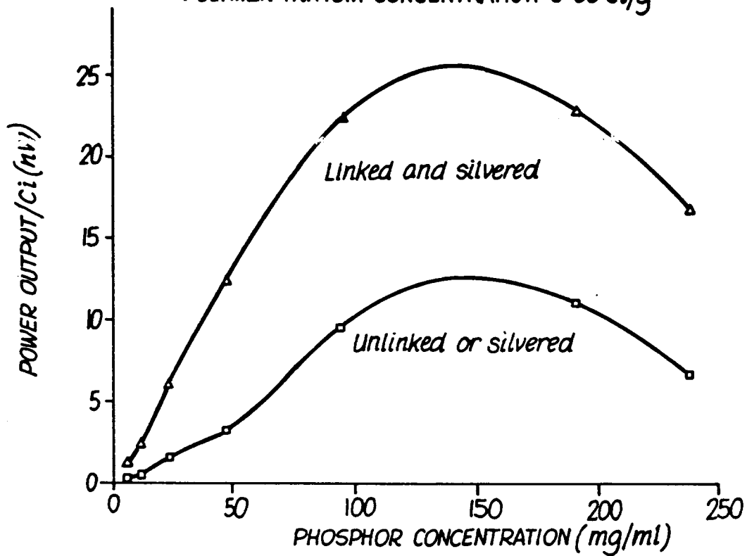
Fig.2. POLYMER TRITIUM CONCENTRATION 6.06 Ci/g
