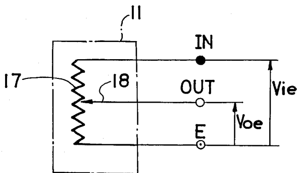
FIGURE 2 PRIOR ART
