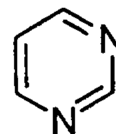
pyrimidine (pyrimidinyl)
