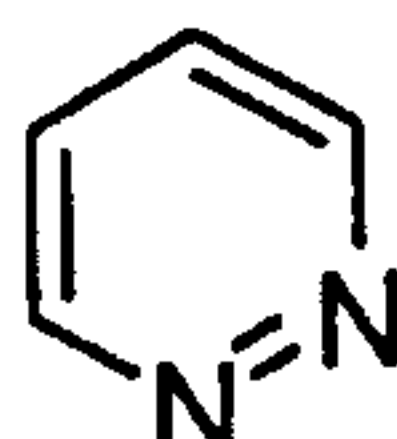
pyridazine (pyridazinyl)
