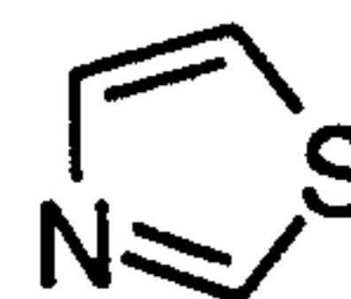
thiazole (thiazolyl)
