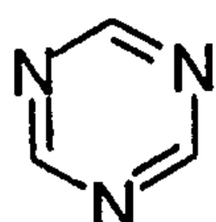
triazine (triazinyl)
