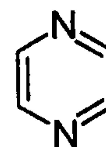
pyrazine (pyrazinyl)
