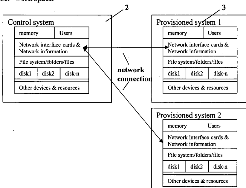
Fig. 5: An example of resource objectives on systems and can be assigned to each group or each user' work space.
