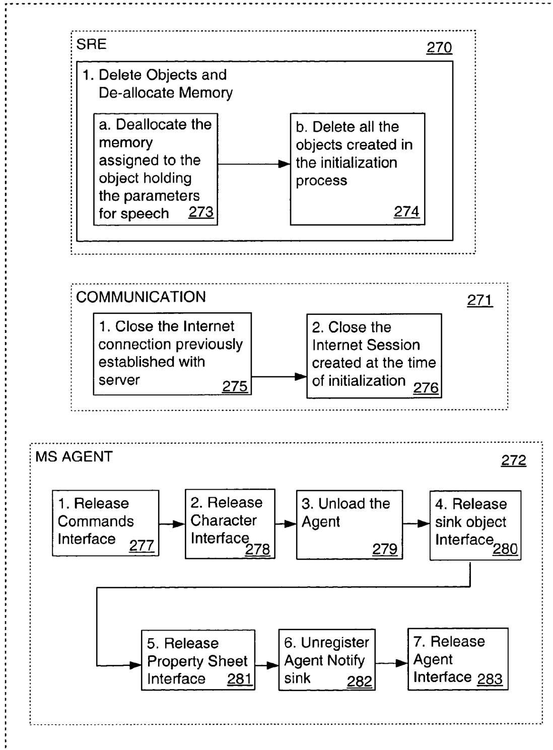
Fig. 4 Client-side Un-Initialization
