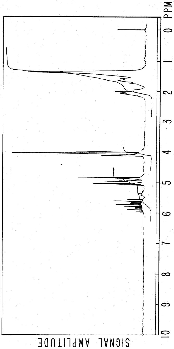
FIG. 1 NMR SPECTRUM FOR EXAMPLE I.
