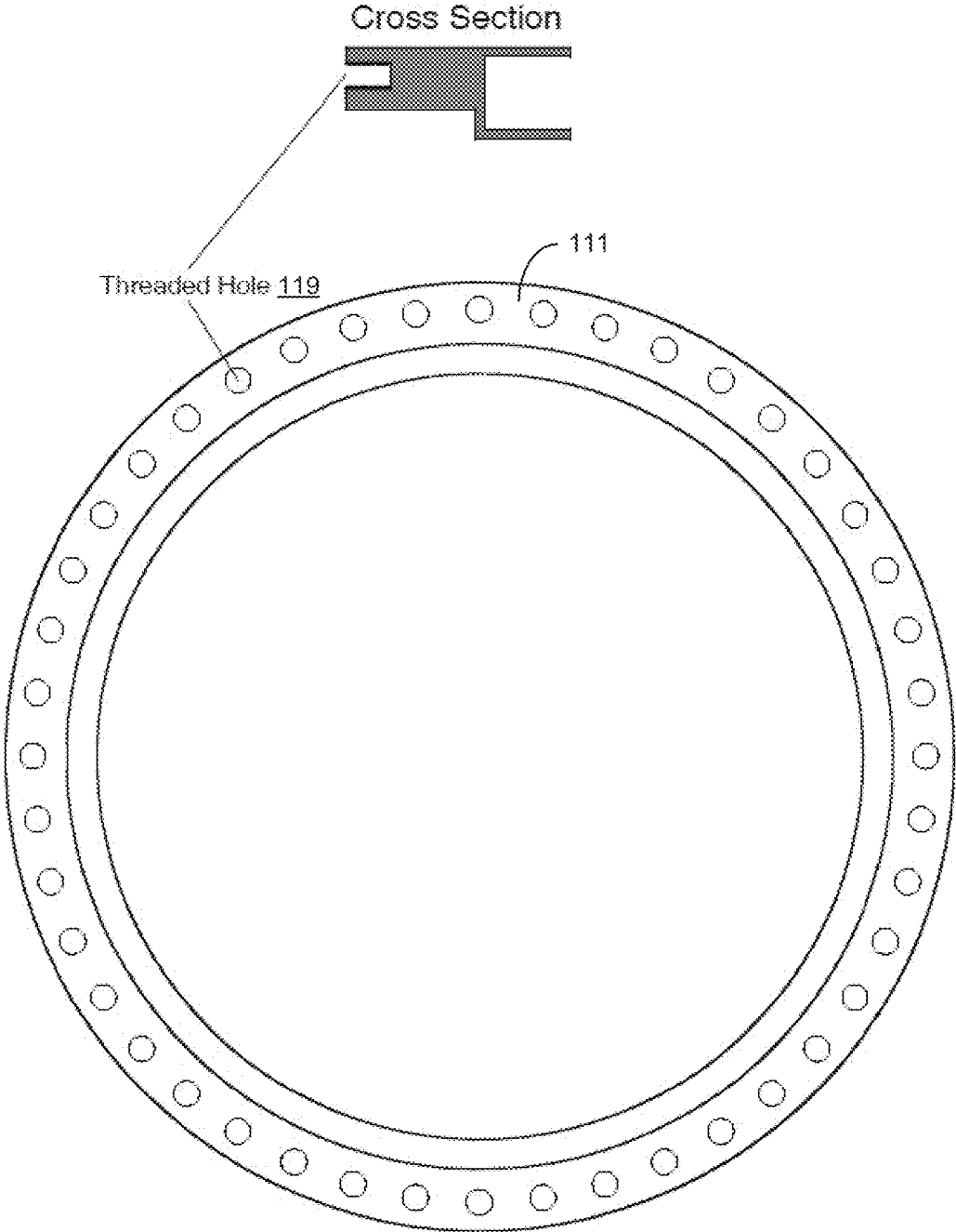
Front View FIG. 3D
