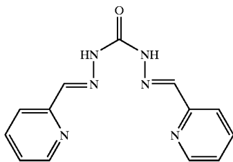
Carbo-Py-Al
