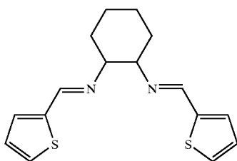
Chxn-Thio-Al
