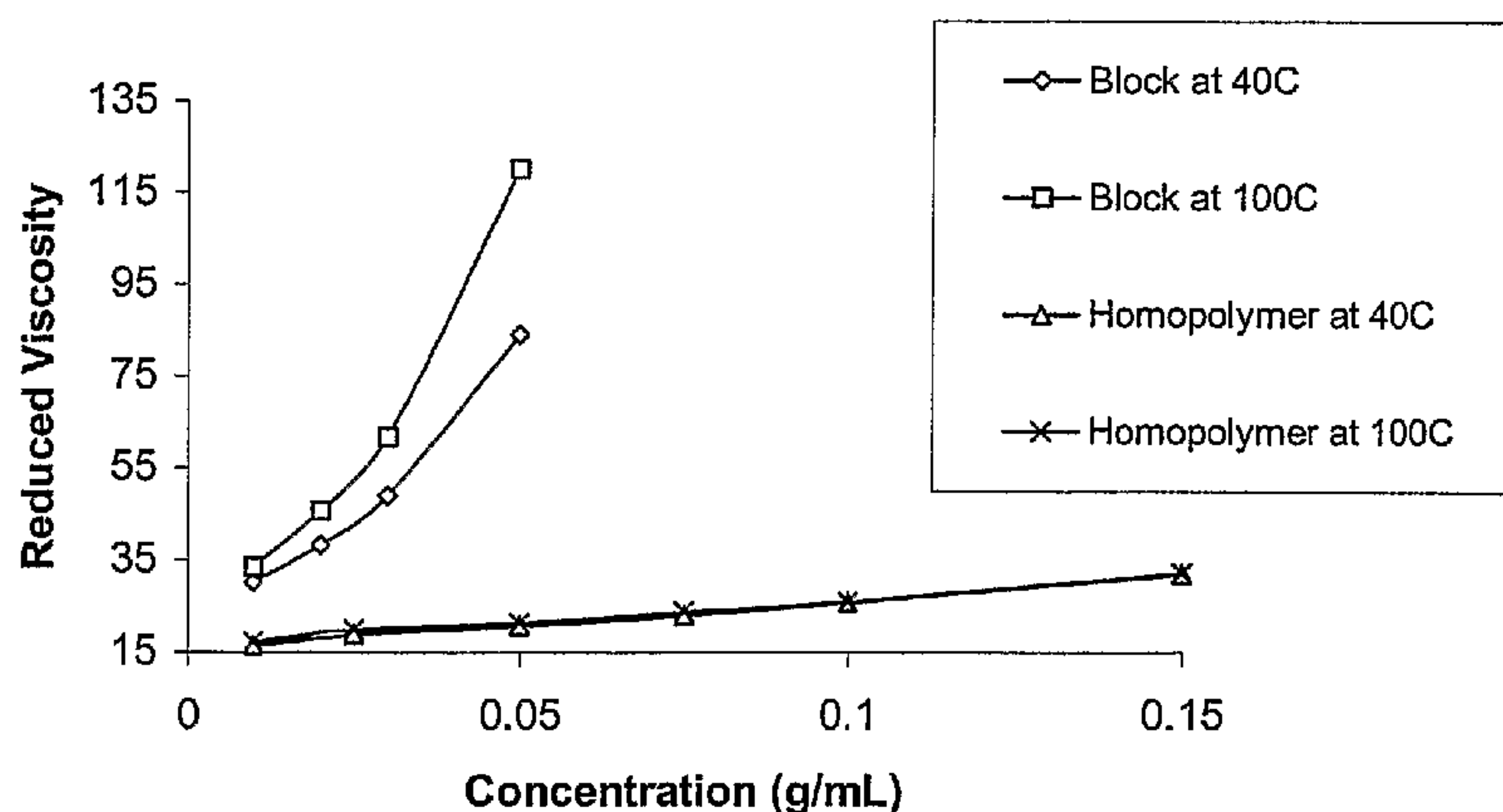
Reduced Viscosity vs. Concentration
