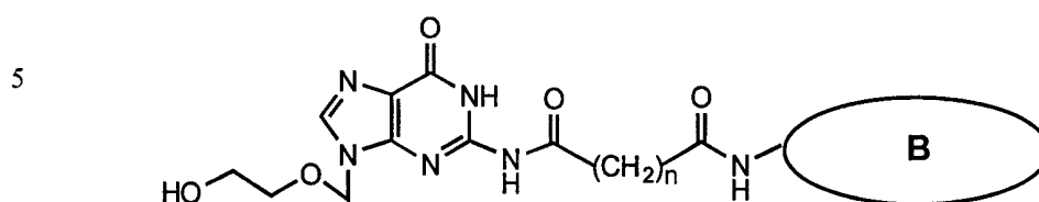
Acyclovir
