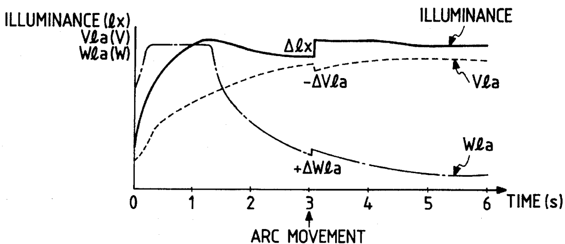
FIG. 15 PRIOR ART
