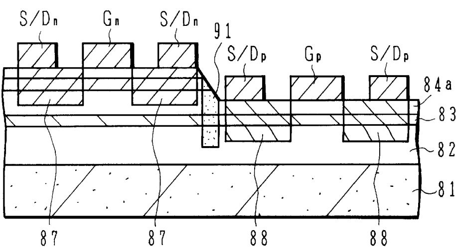
FIG.8C (PRIOR ART)
