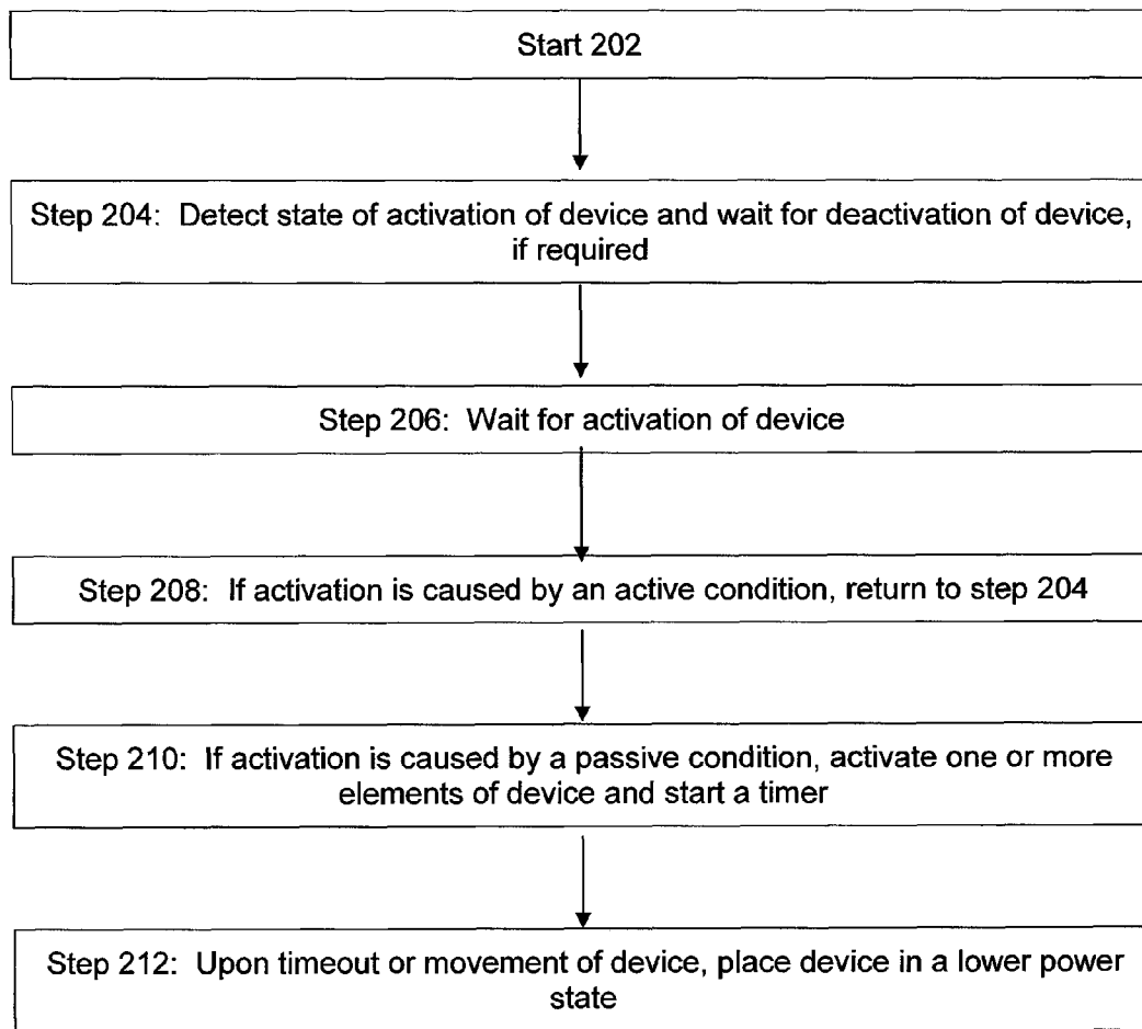
Algorithm 200
