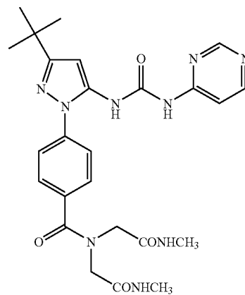
Example 57
