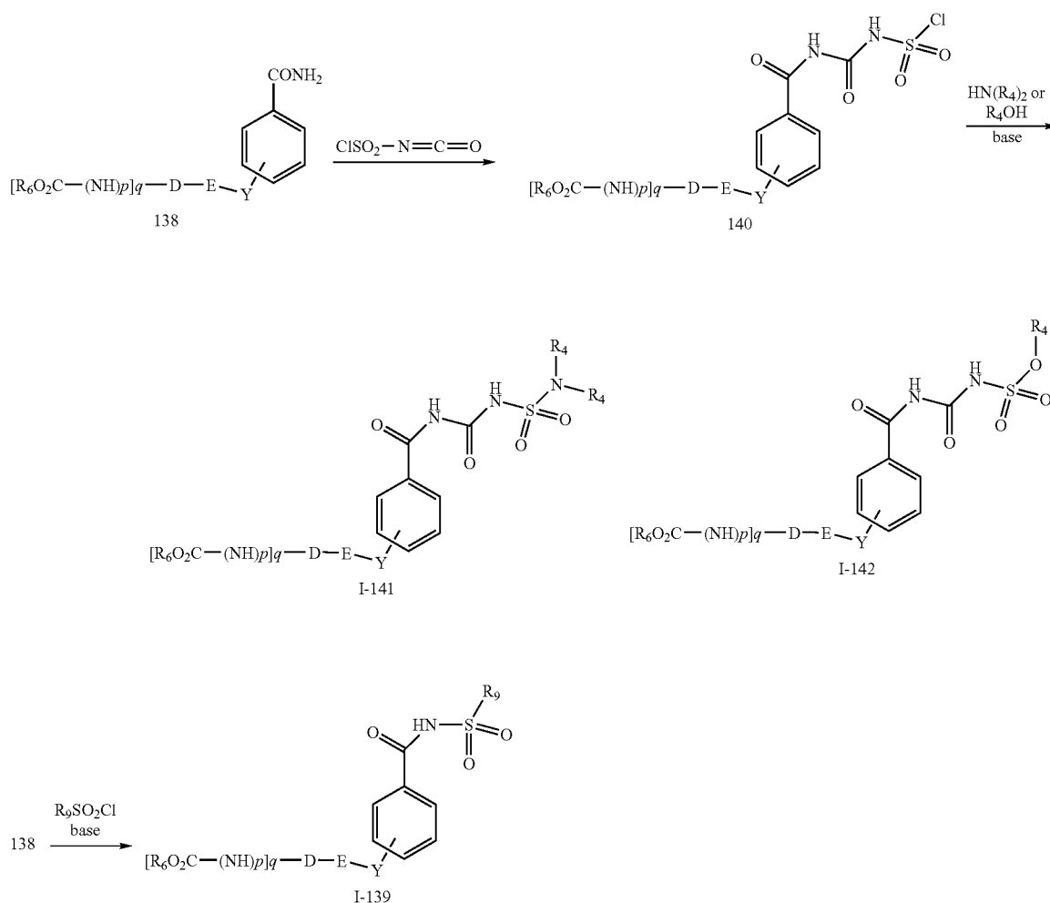
Scheme 22
