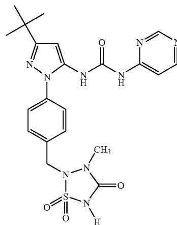
Example 15
