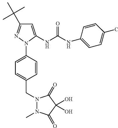
Example 32
