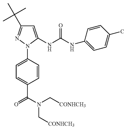
Example 56
