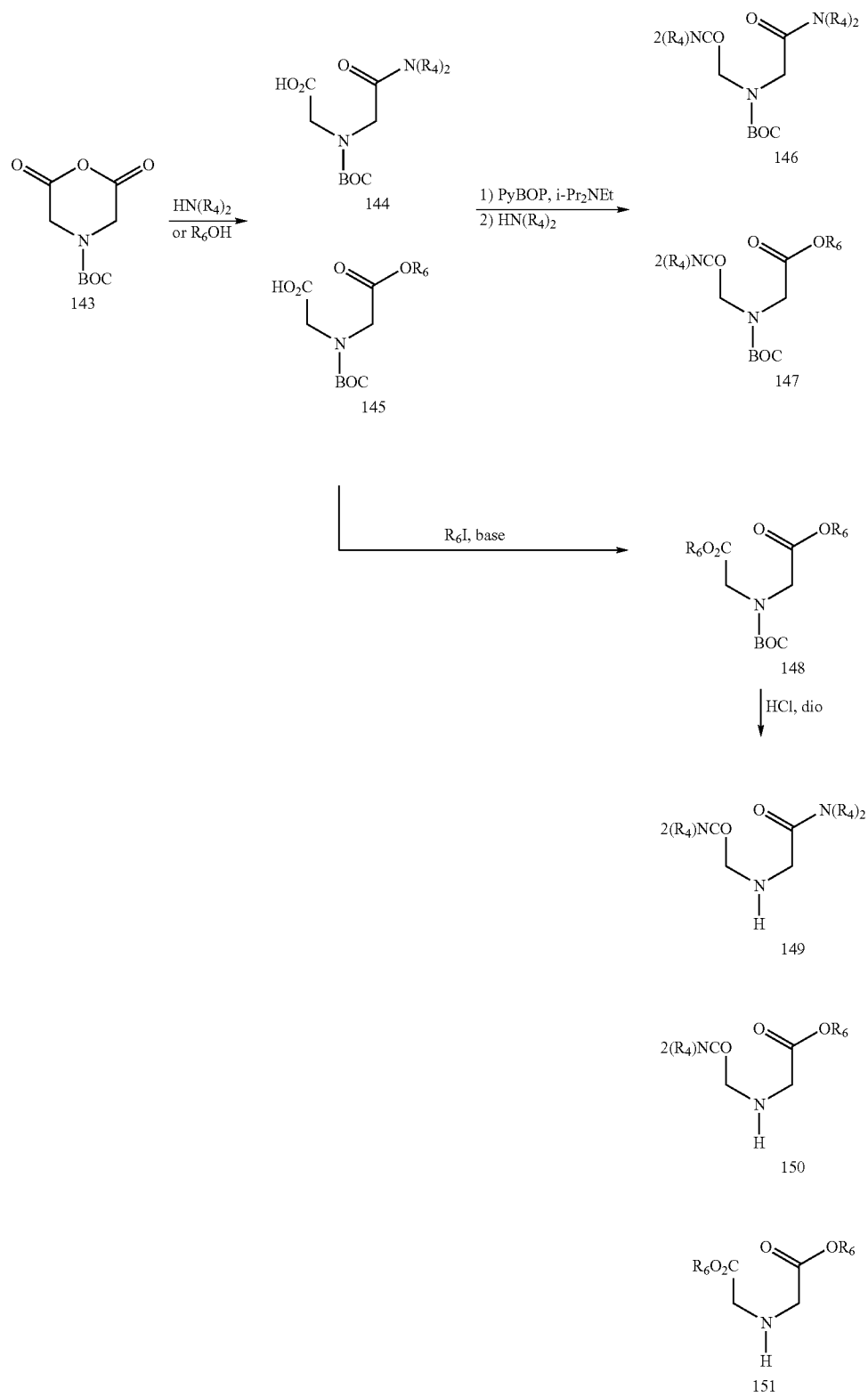
Scheme 23
