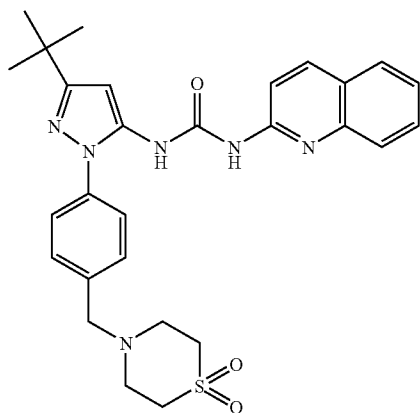
Example 48
