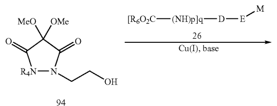
Scheme 16.2
