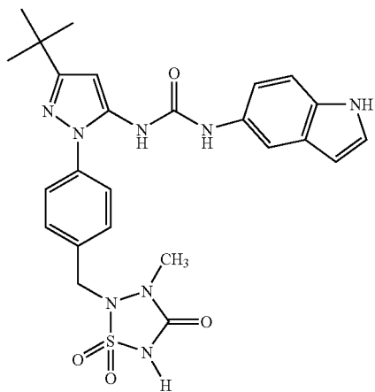
Example 18
