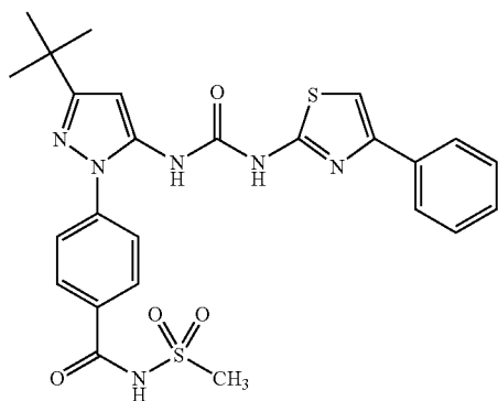
Example 53
