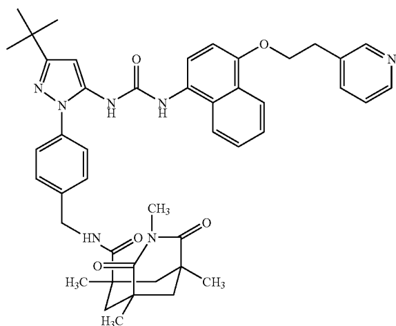
Example 114
