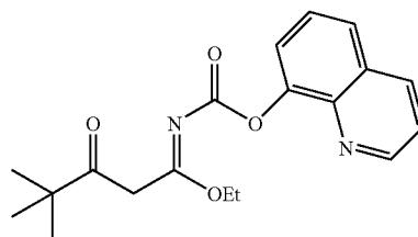
Example MM
