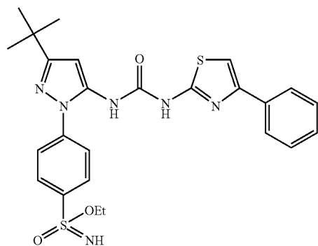
Example 71
