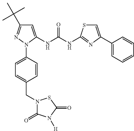
Example 11
