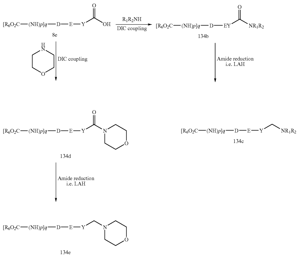
Scheme 21.2
