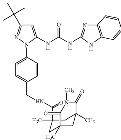
Example 39
