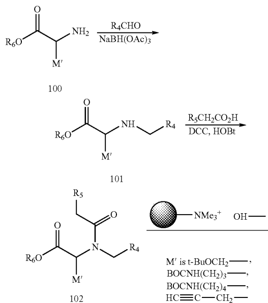
Scheme 17.1
