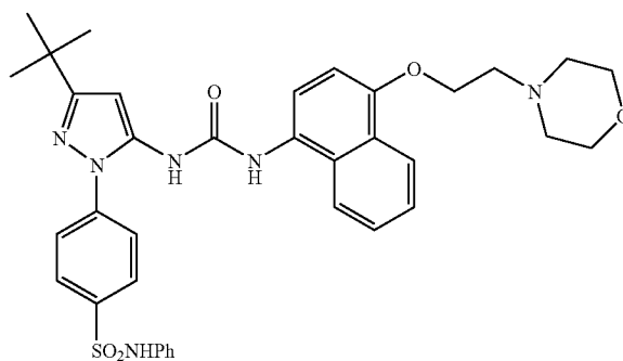
Example 134
