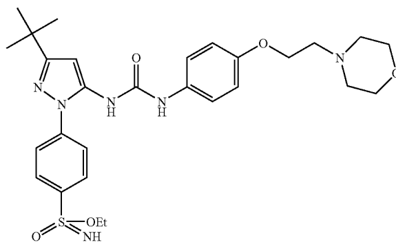
Example 141
