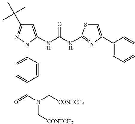
Example 59
