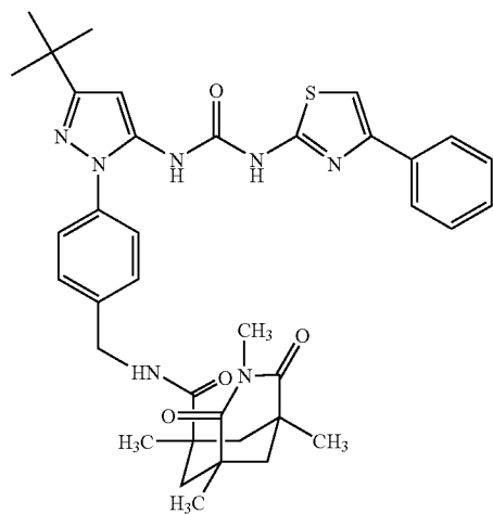
Example 41
