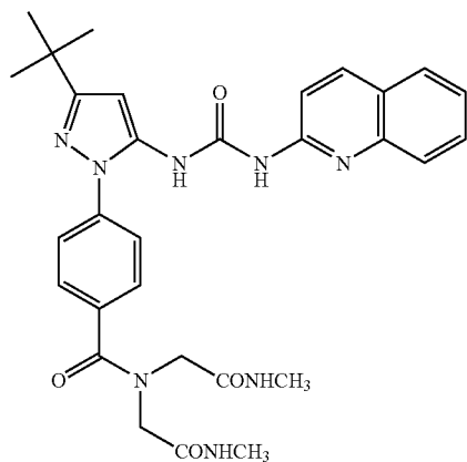
Example 60
