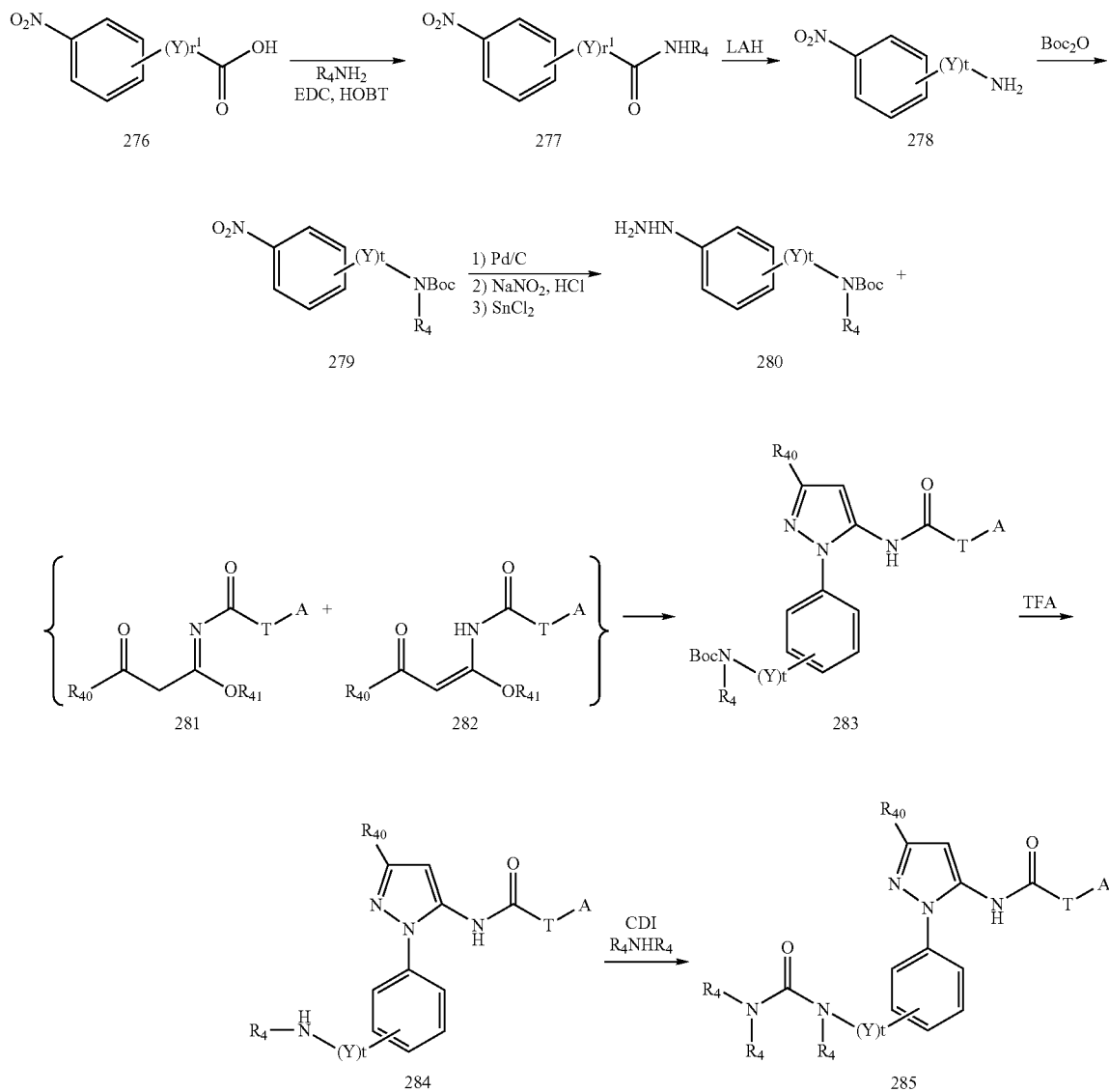
Scheme 52
