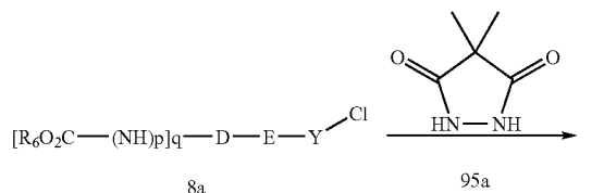
Scheme 16.3
