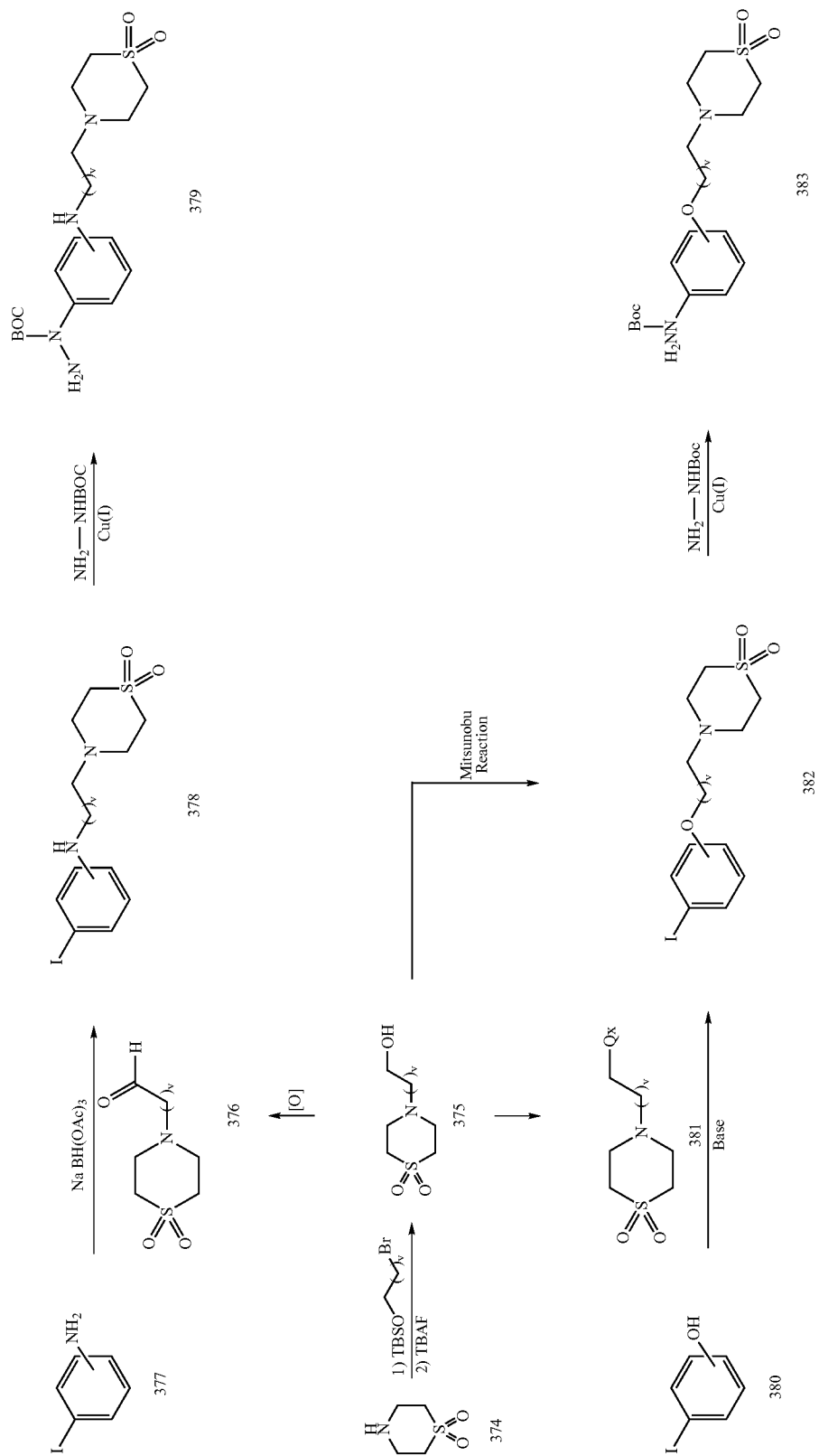
Scheme 67
