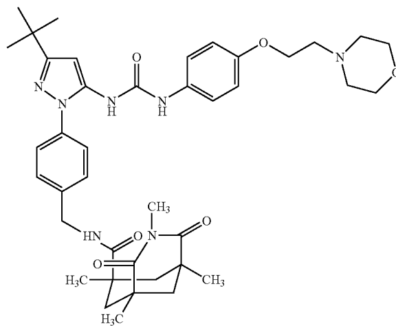
Example 111
