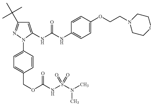
Example 99
