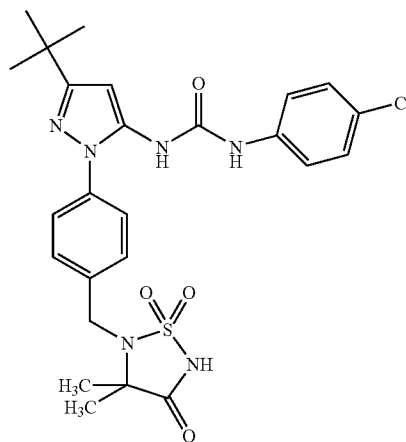
Example 20
