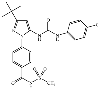
Example 50
