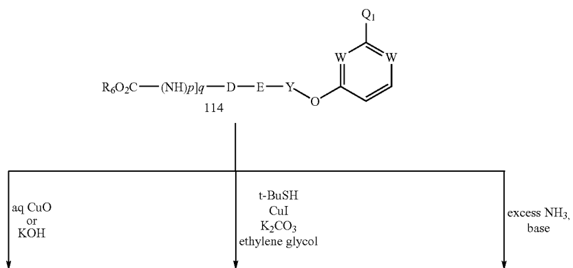
Scheme 19.3
