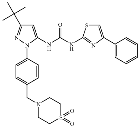
Example 47
