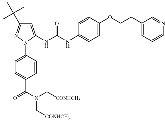
Example 132
