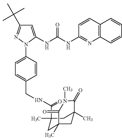
Example 42
