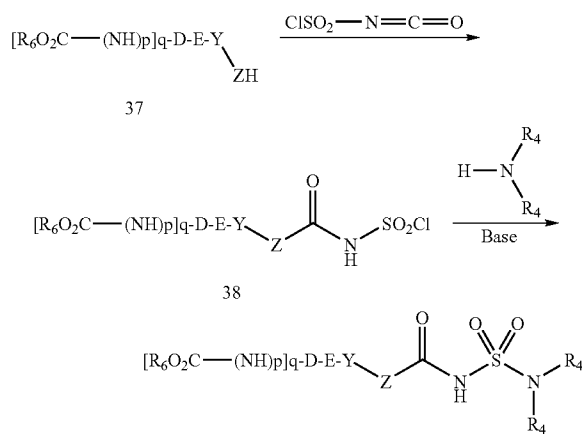
Scheme 7.2
