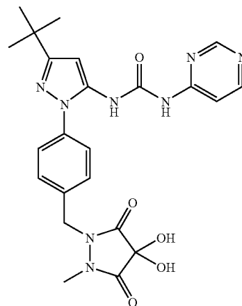
Example 33
