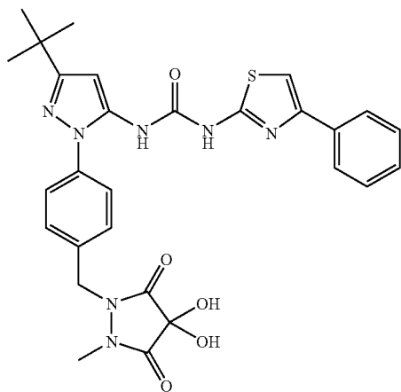
Example 35
