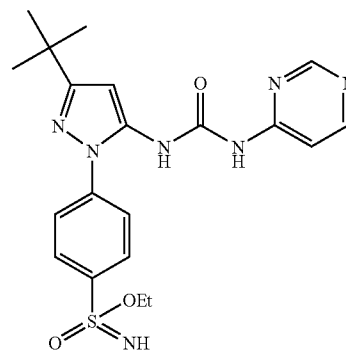
Example 69
