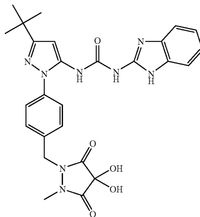
Example 33
