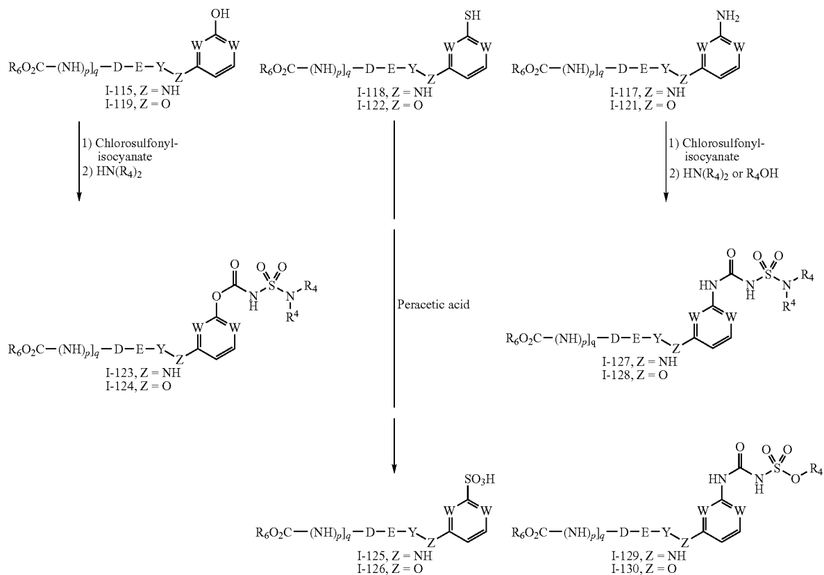
Scheme 20
