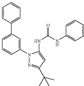
Example 33
