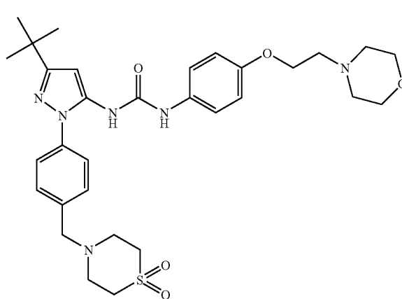
Example 117
