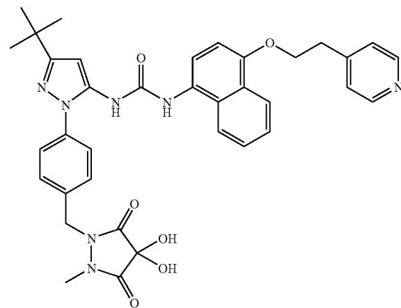
Example 105
