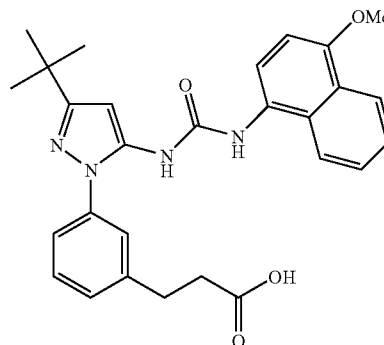
Example 175
