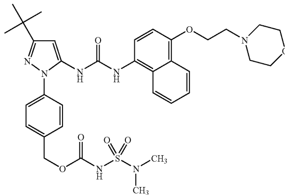
Example 98
