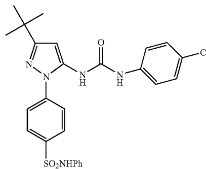
Example 62
