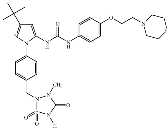
Example 87
