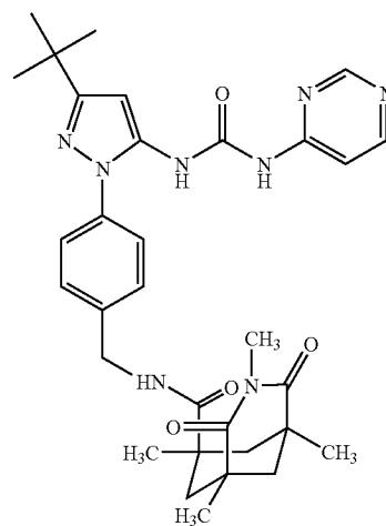
Example 39
