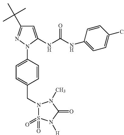
Example 14
