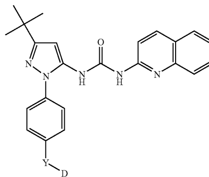
Example 6
