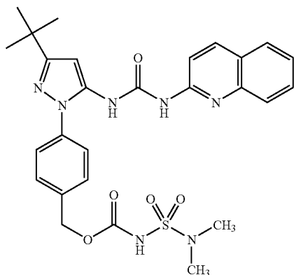
Example 30
