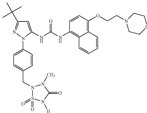
Example 86
