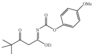
Example LL
