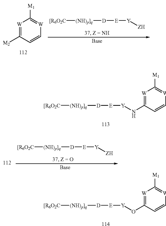
Scheme 19.1
