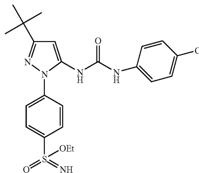
Example 68
