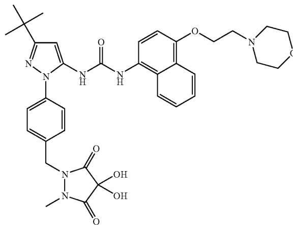
Example 104
