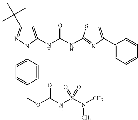
Example 29
