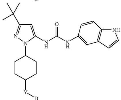
Example 2
