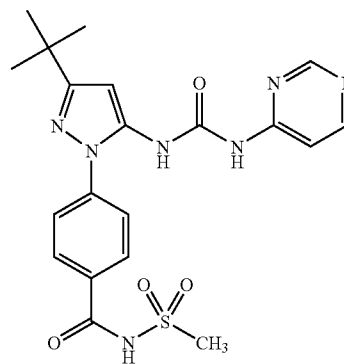
Example 51
