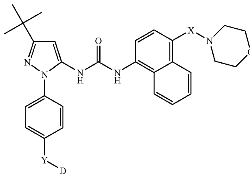
Example 74
