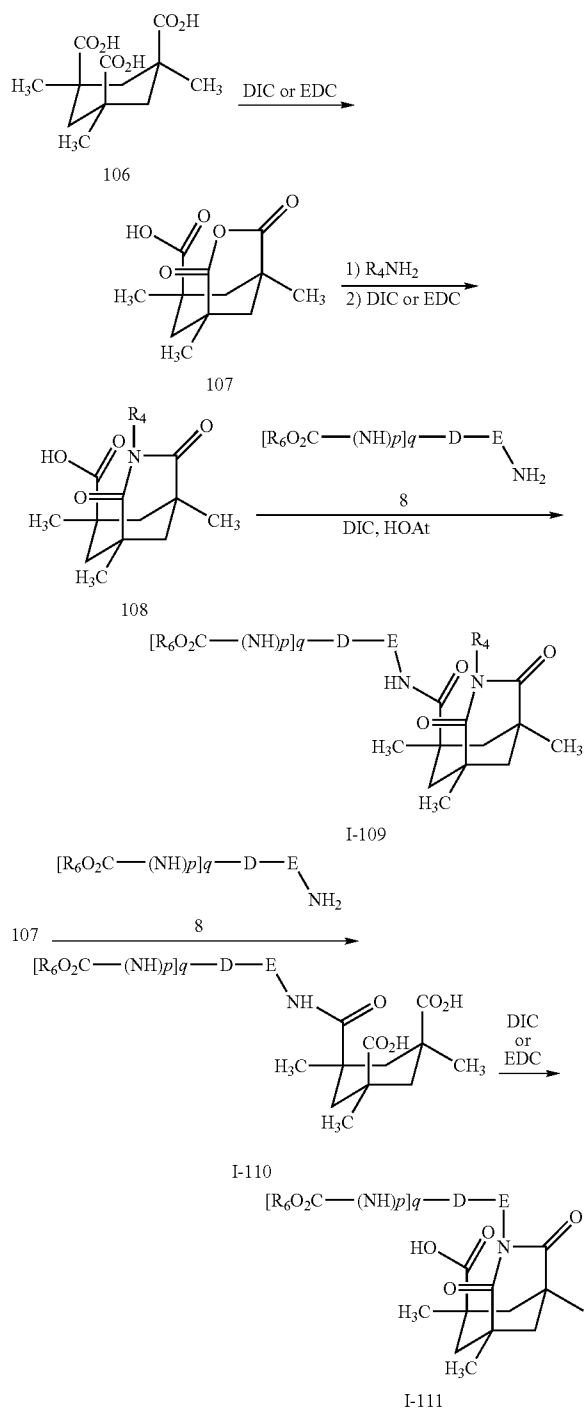
Scheme 18
