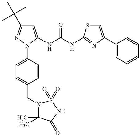
Example 23
