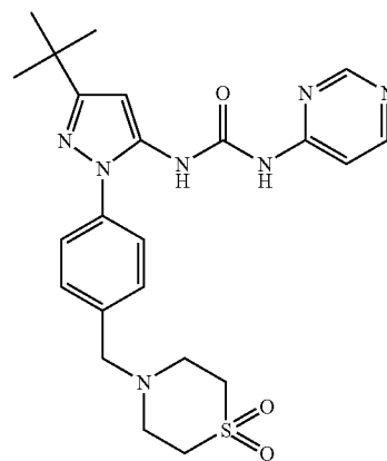
Example 45
