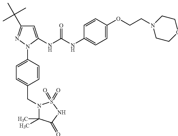
Example 93
