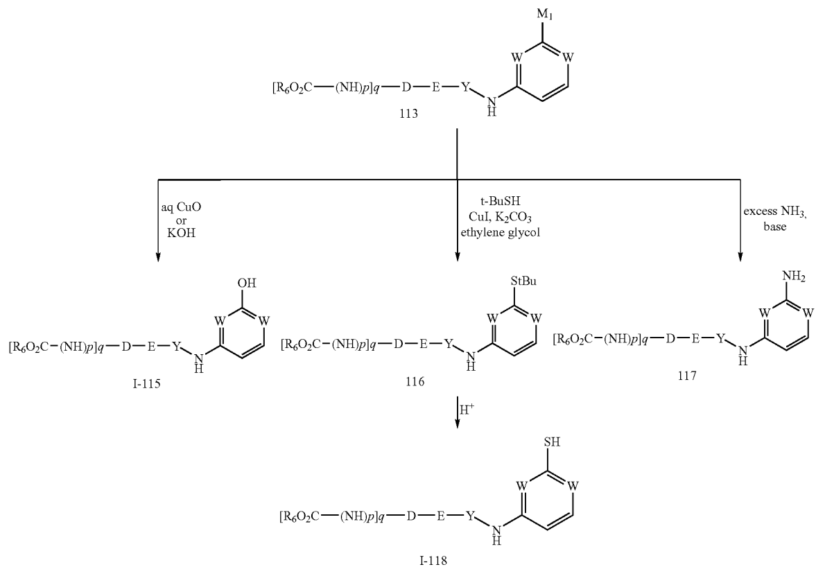
Scheme 19.2
