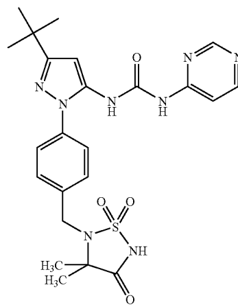
Example 21
