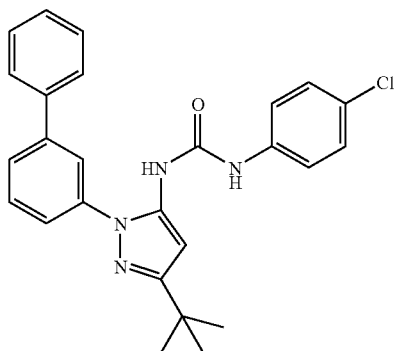
Example 34
