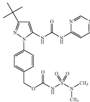
Example 27
