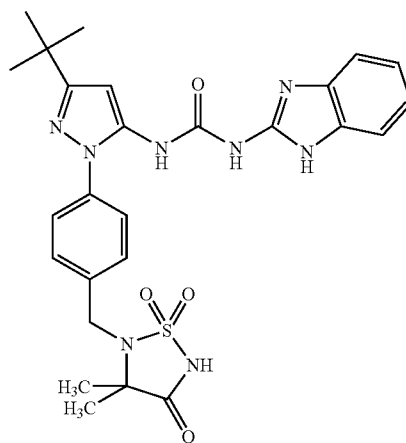
Example 21
