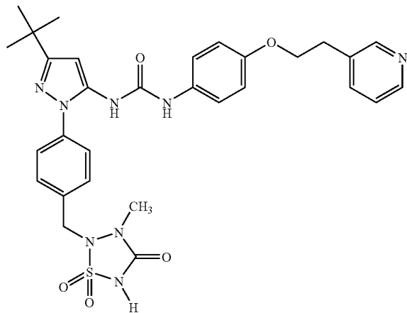
Example 90
