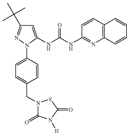
Example 12
