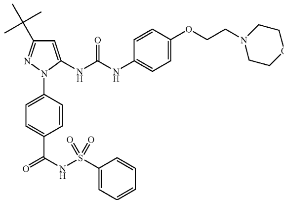
Example 123
