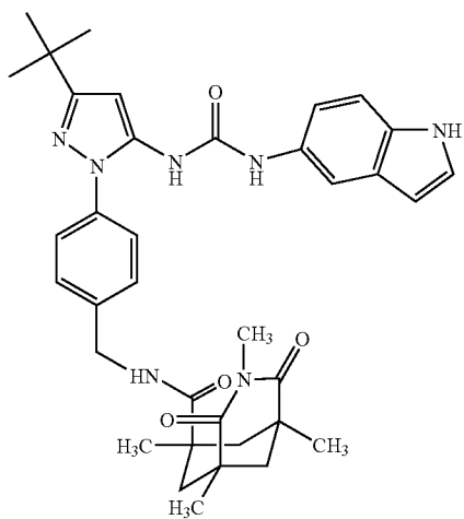
Example 42
