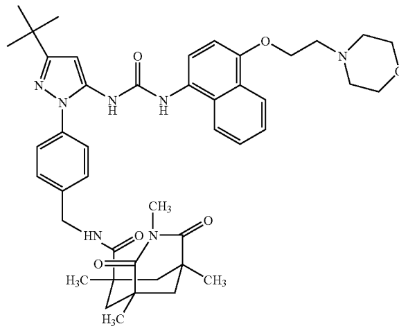
Example 110
