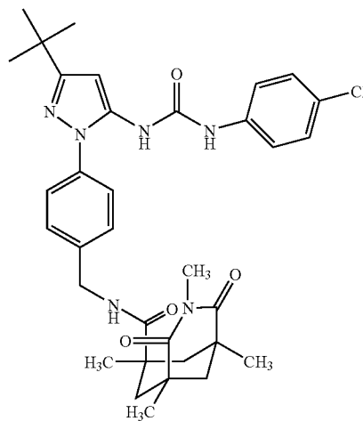
Example 38
