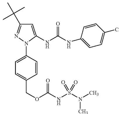
Example 26
