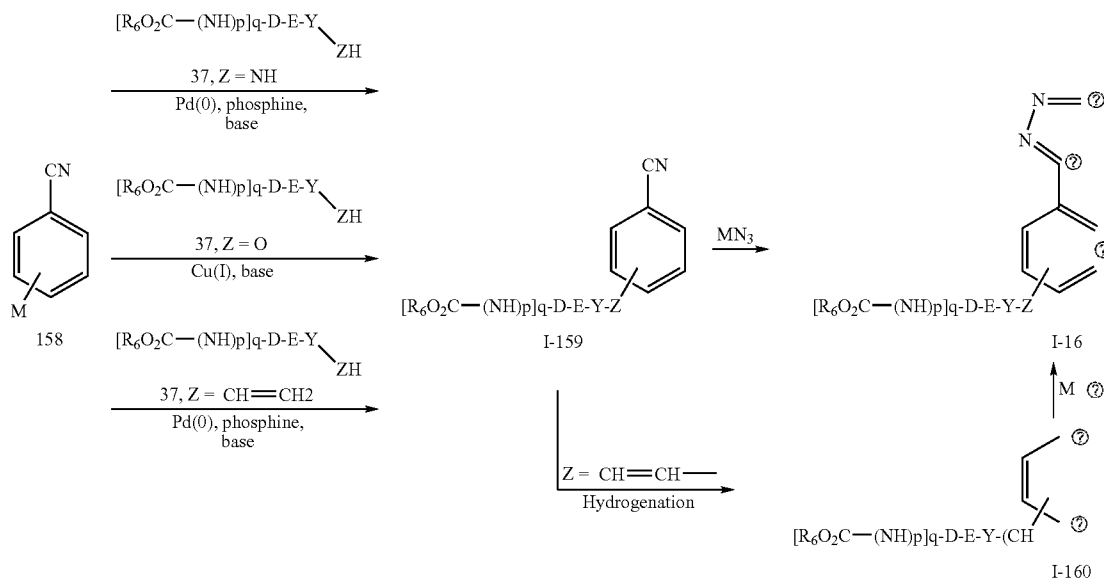
Scheme 25
