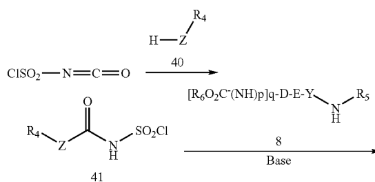
Scheme 7.2
