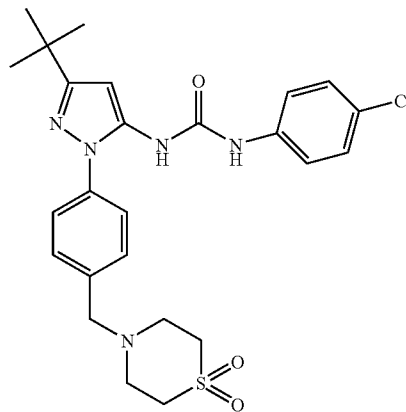
Example 44
