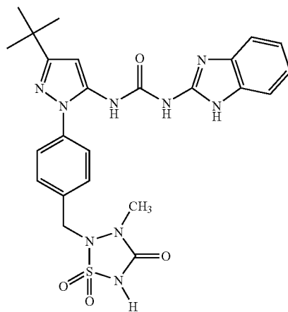
Example 15
