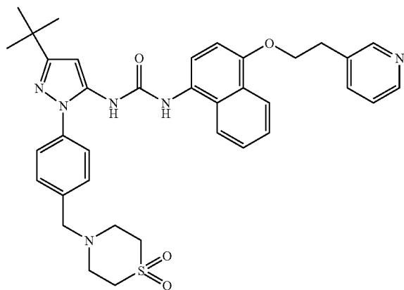
Example 120
