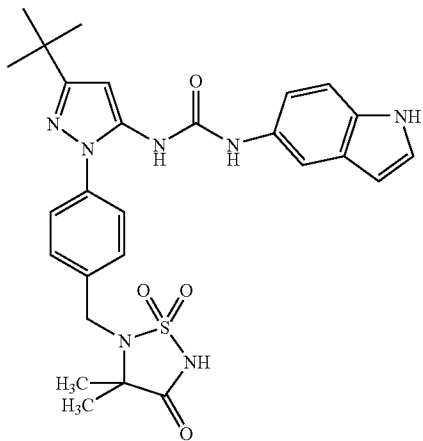
Example 24
