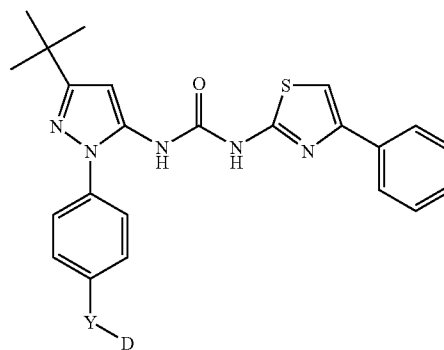
Example 5
