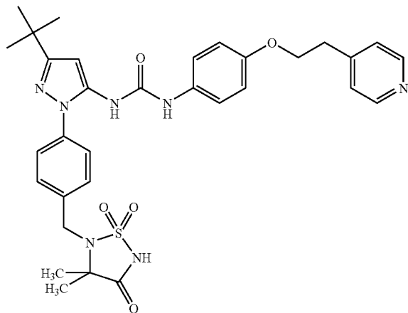
Example 94
