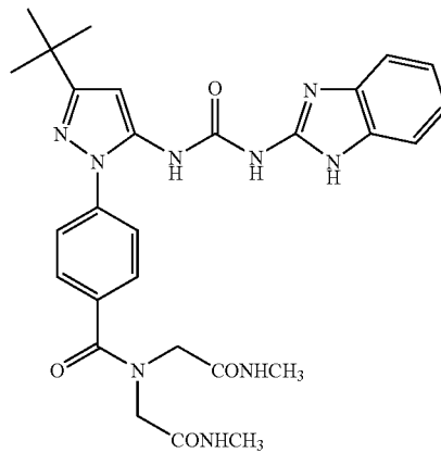
Example 57
