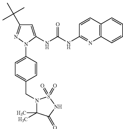
Example 24
