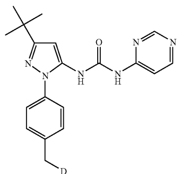
Example 3
