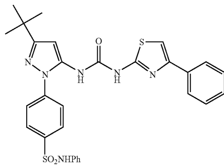
Example 65
