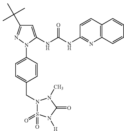
Example 18
