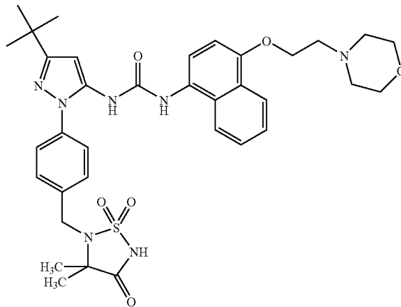
Example 92
