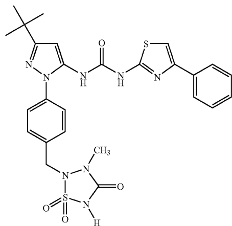
Example 17
