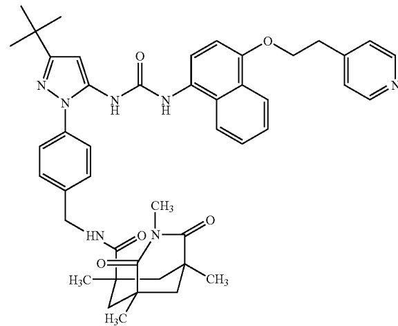
Example 111
