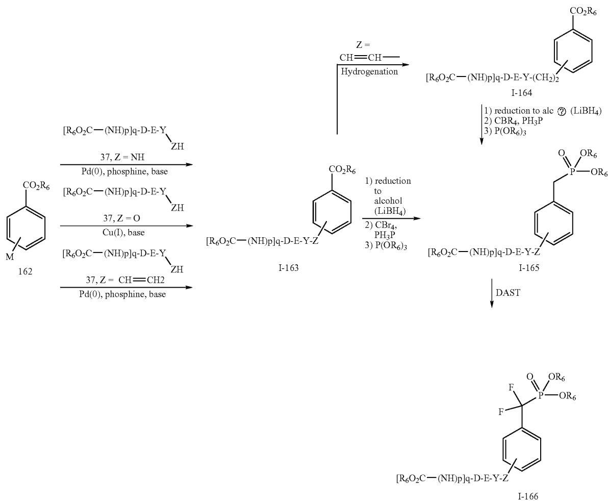
Scheme 26
