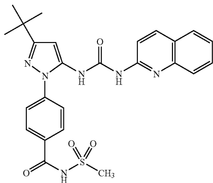
Example 54
