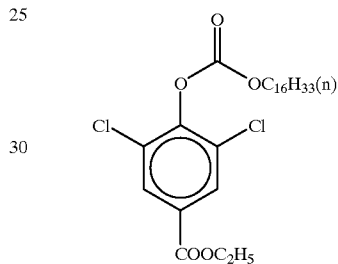
(ExC-2) Cyan Coupler
