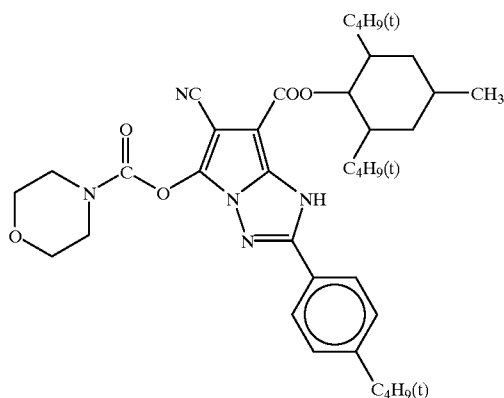
(ExC-2) Cyan Coupler
