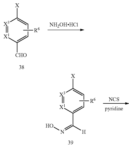
Scheme 7
