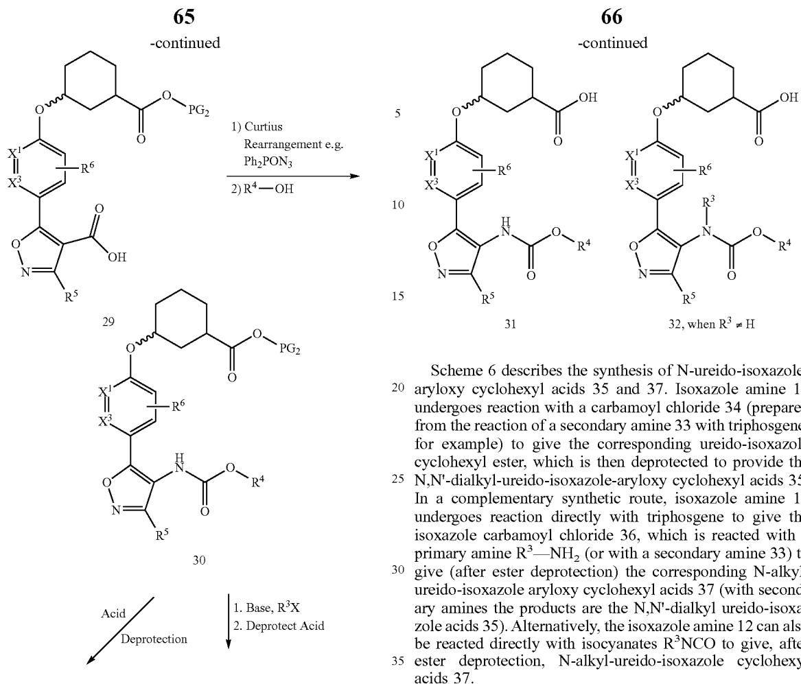
Scheme 6
