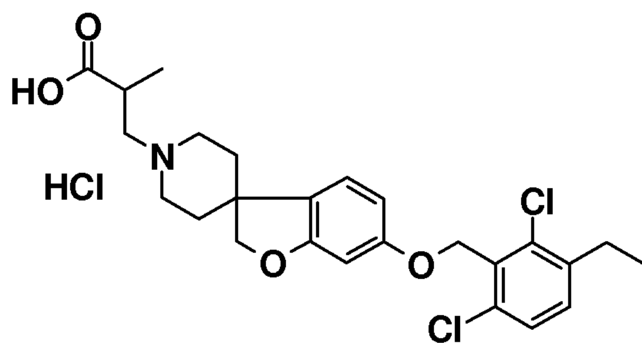
Compound 99. 3-{6-[(2,6-Dichloro-3-ethylphenyl)methoxy]-2H-
