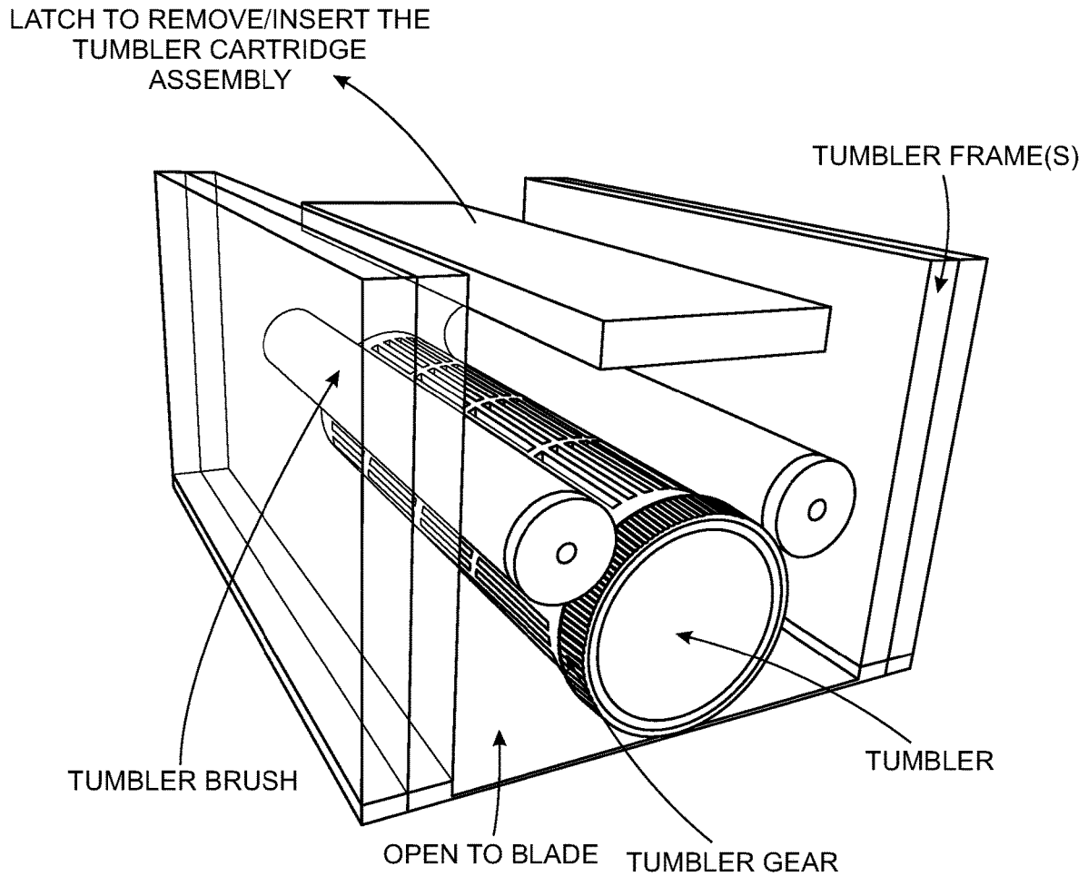
TUMBLER ASSEMBLY - BACK VIEW
