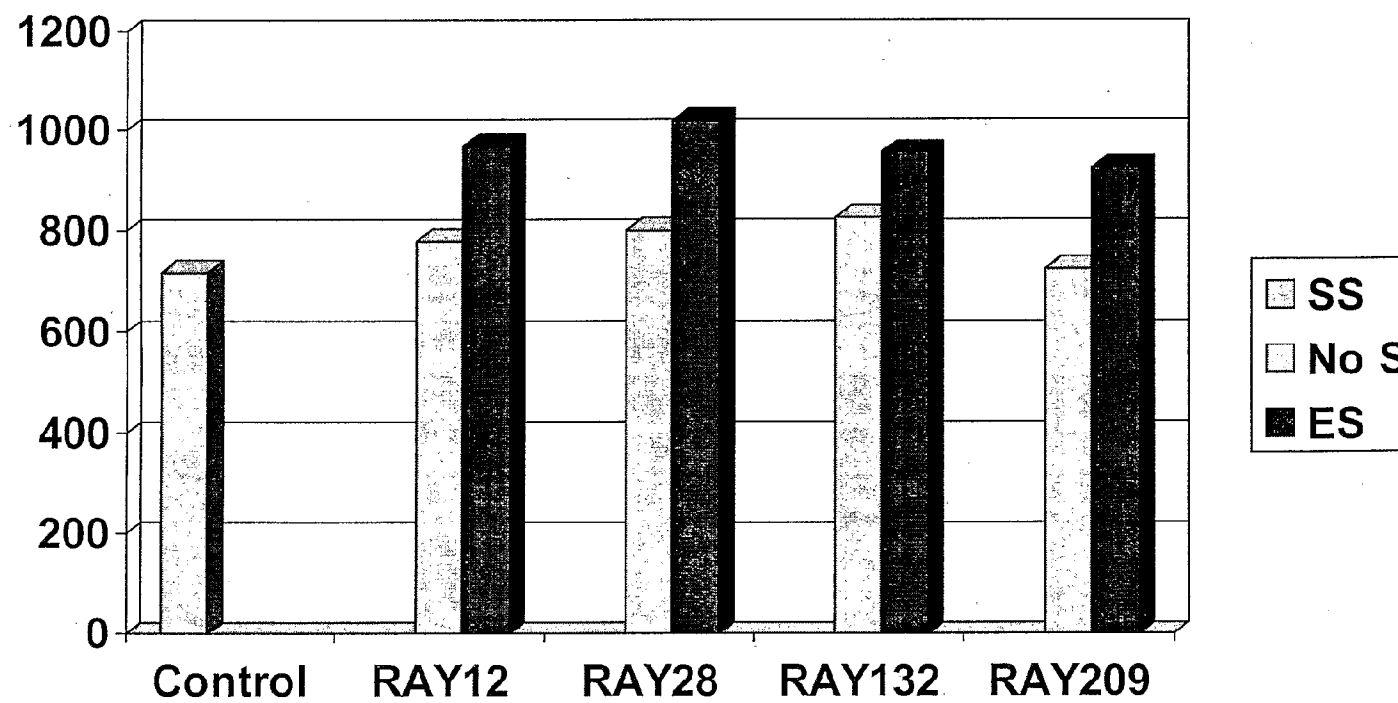
Figure 6. Canola yield (kg/ha) in 2001 field trial in Miami, MB
