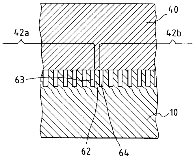
FIG. 5B SECTION C-C
