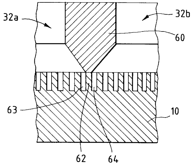
FIG. 5A SECTION B-B
