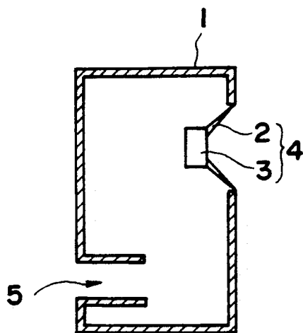
FIG. 6 PRIOR ART
