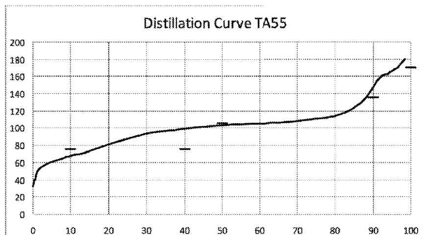
Distillation curve of TA-55
