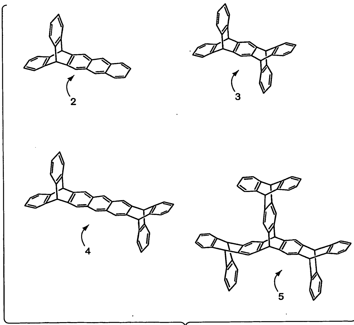
Fig. 1C (PRIOR ART)
