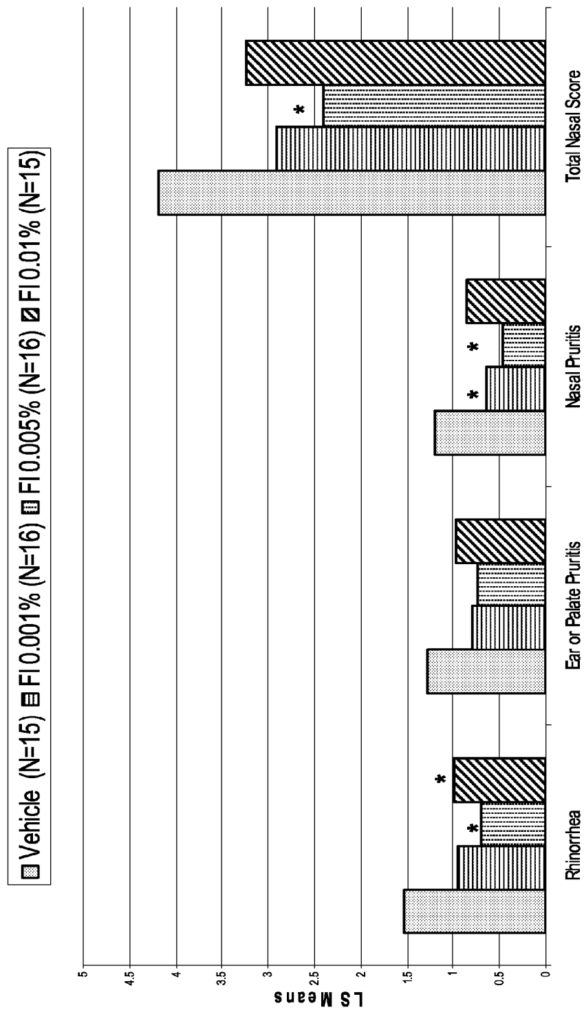
Figure 18: ANCOVA Nasal
