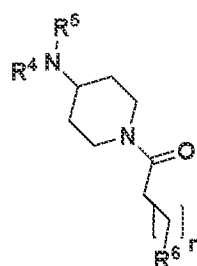
(Ic)
