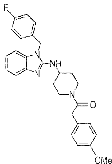
Acyl Astemizole (2)
