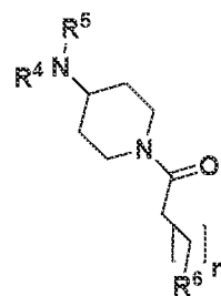
(Ic)
