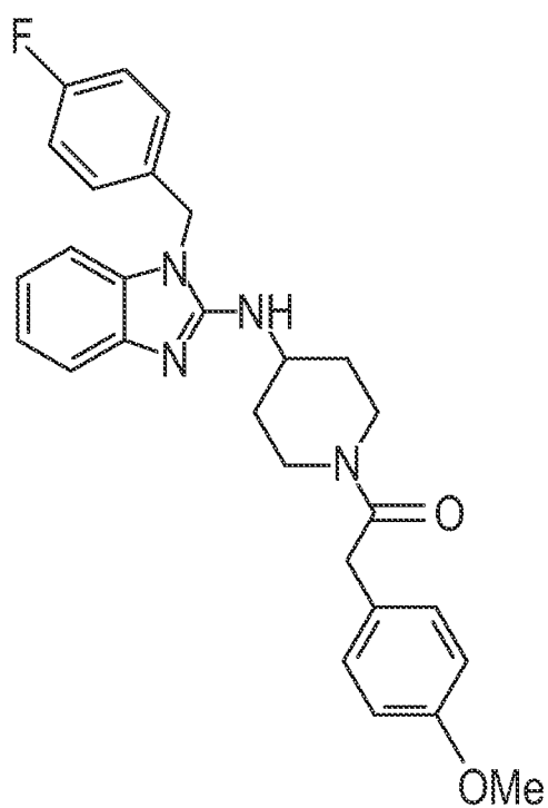
Acyl Astemizole (2)
