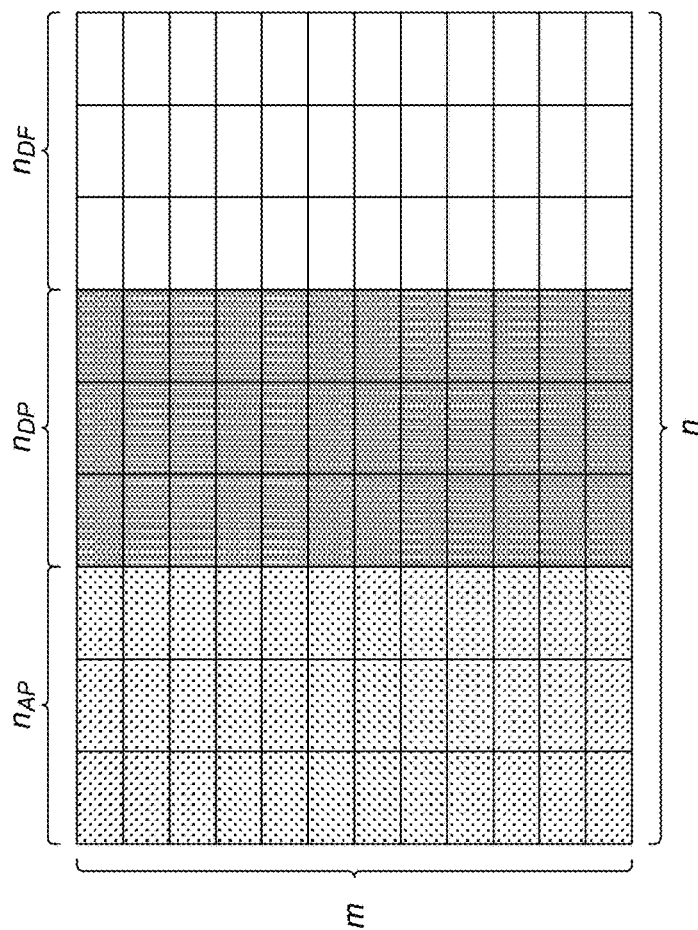
Example Training Matrix X
