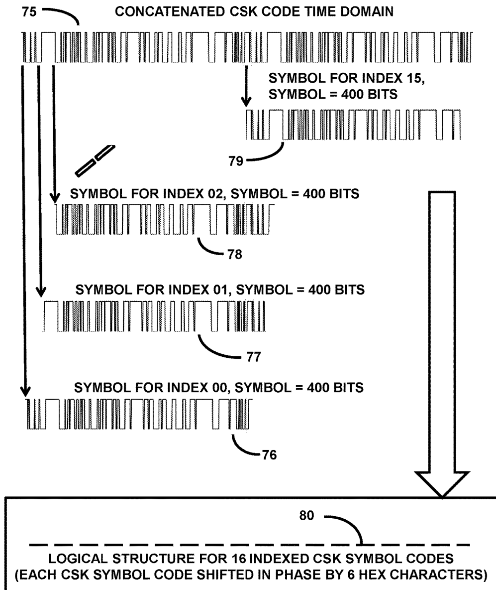
FIG. 6 A MEANS FOR EXTRACTION OF 16 ORTHOGONAL CSK SYMBOL CODES PROVIDED TO SUPPORTED SIGNAL PROCESSING SYSTEMS THAT SYNCHRONOUSLY RECEIVE ORIGINAL CSK CODES FROM MEMORY
