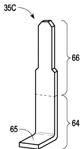
POST ELECTRICAL PRESS-FIT TERMINAL
