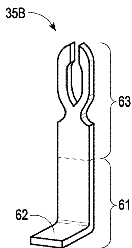
FORK ELECTRICAL PRESS-FIT TERMINAL
