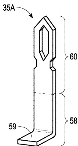
EYE-OF-THE-NEEDLE ELECTRICAL PRESS-FIT TERMINAL
