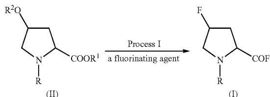
Scheme 4; Process I
