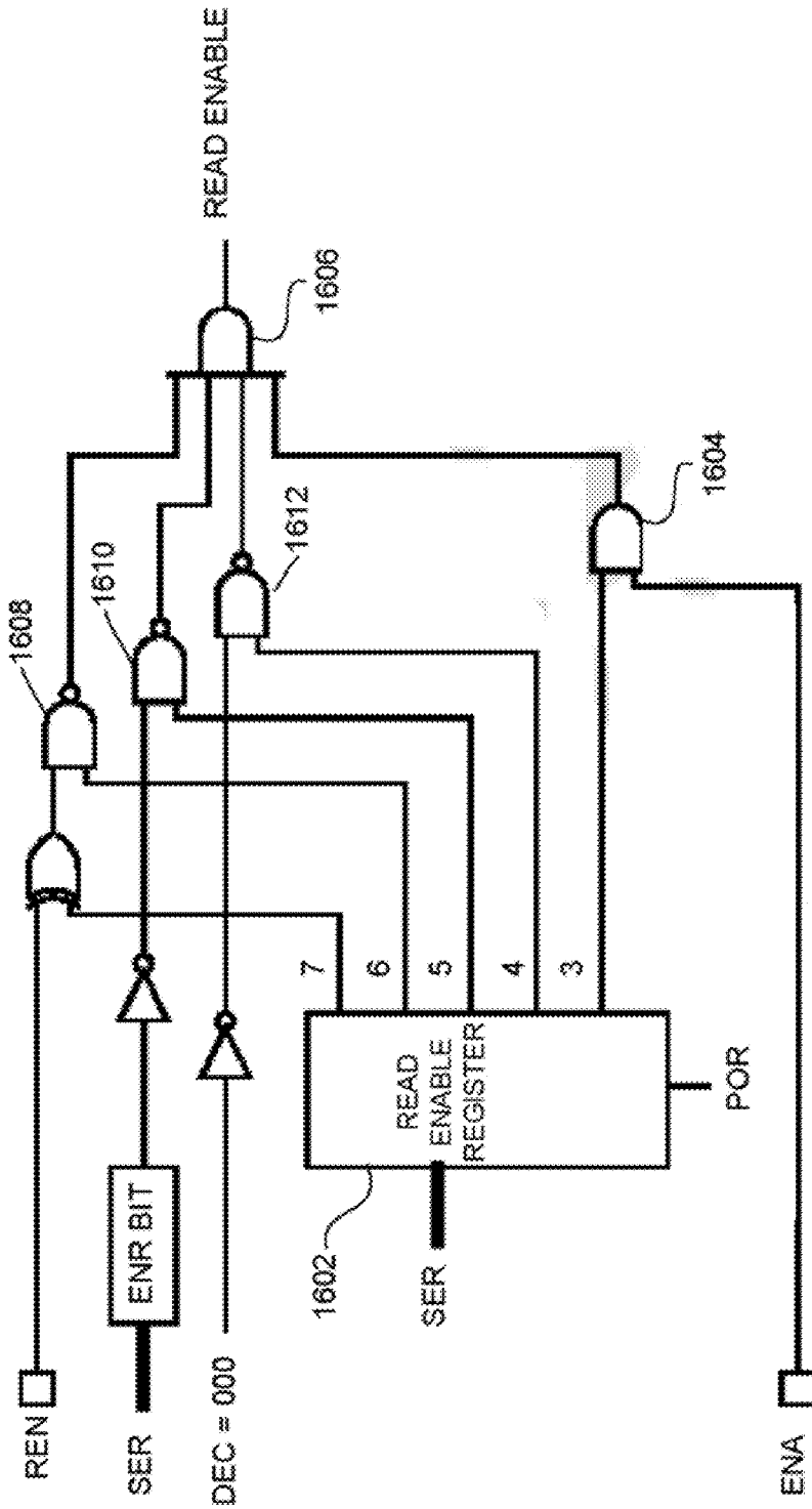
SERIAL CONFIGURABLE READ ENABLE LOGIC
