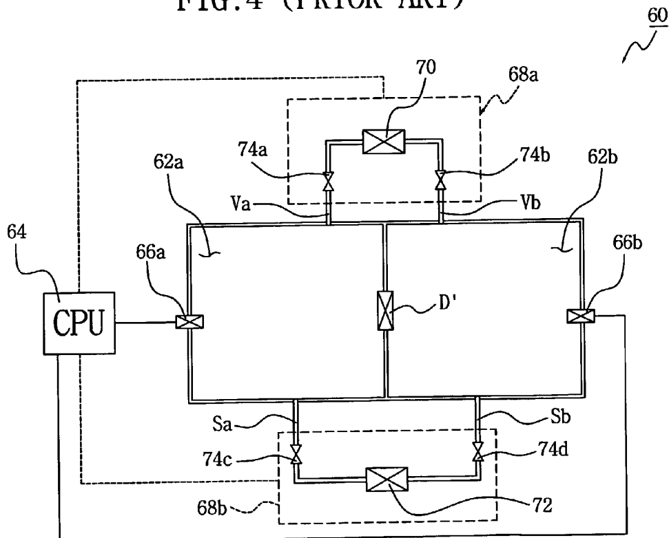
FIG. 4 (PRIOR ART)
