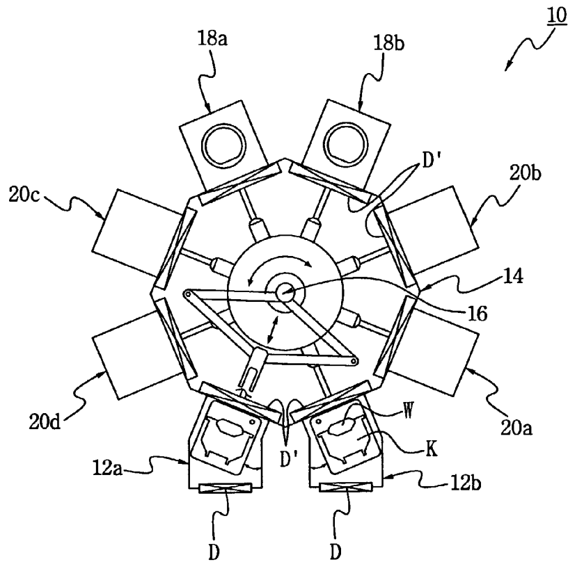
FIG. 2 (PRIOR ART)
