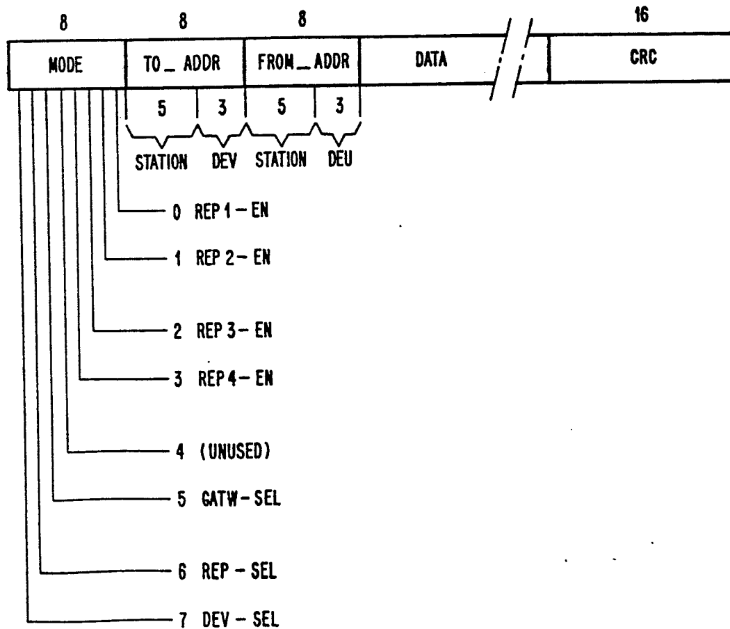
FIG. 7 PACKET FORMAT
